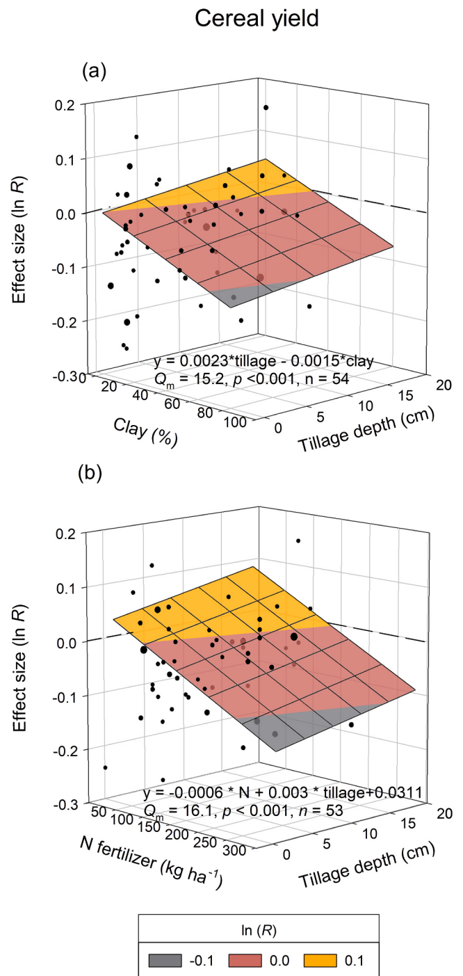
Fig. 4. Combined effects of (a) tillage depth in conservation agriculture and topsoil clay content and (b) tillage depth and mineral N fertilizer on the relative yield ( \ln R ). The doses of mineral N fertilizer are similar in conventional agriculture (CONV) and conservation agriculture. Symbol size corresponds to study weight. The dashed horizontal line indicates CONV. Q_m , model heterogeneity, and n is the number of independent studies. Note that the clay content was documented in 54 studies, whereas the quantity of N fertilizer was reported in 53 studies.
