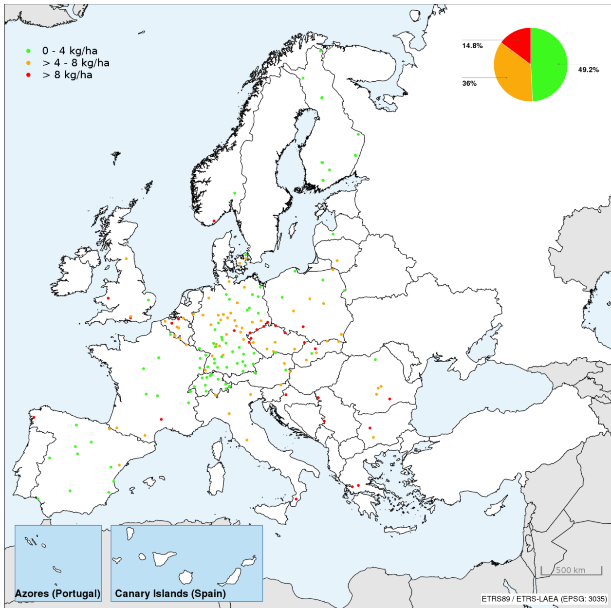
Figure 4-5. Throughfall atmospheric deposition of sulphate sulphur ( \text{SO}_4\text{-S} ) in European forests in 2014.
