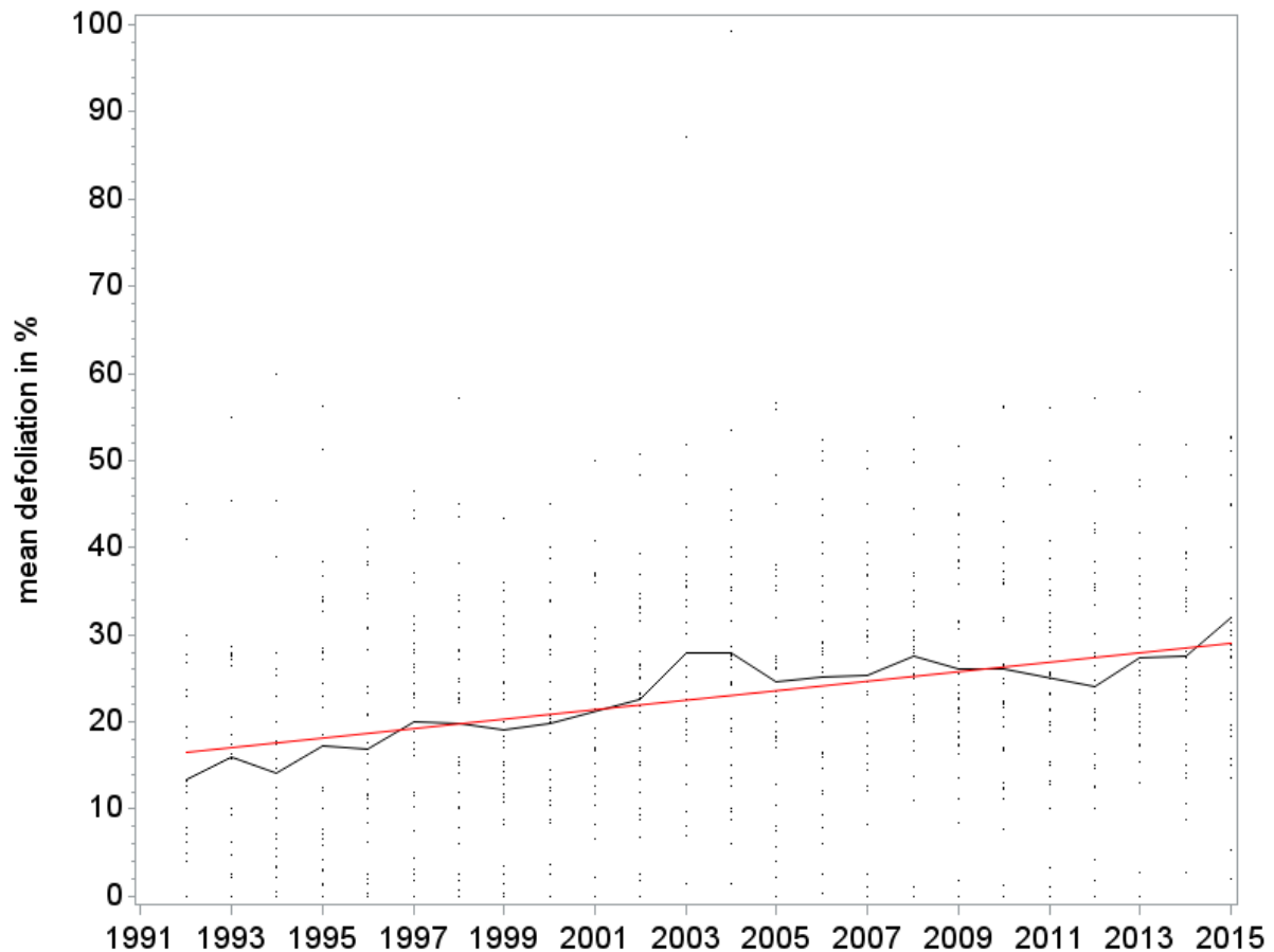
Figure 3-9. Over-all trend (regional Sen's slope = 0.5, p < 0.001 ; minimum length of time span: 20 years, red line) and yearly over-all mean defoliation (black line) of Austrian pine at Level I sites in France, Italy, Hungary, Romania, Bulgaria, Croatia and Belgium; points represent annual plot means, for clarity these are not interconnected from year to year.
