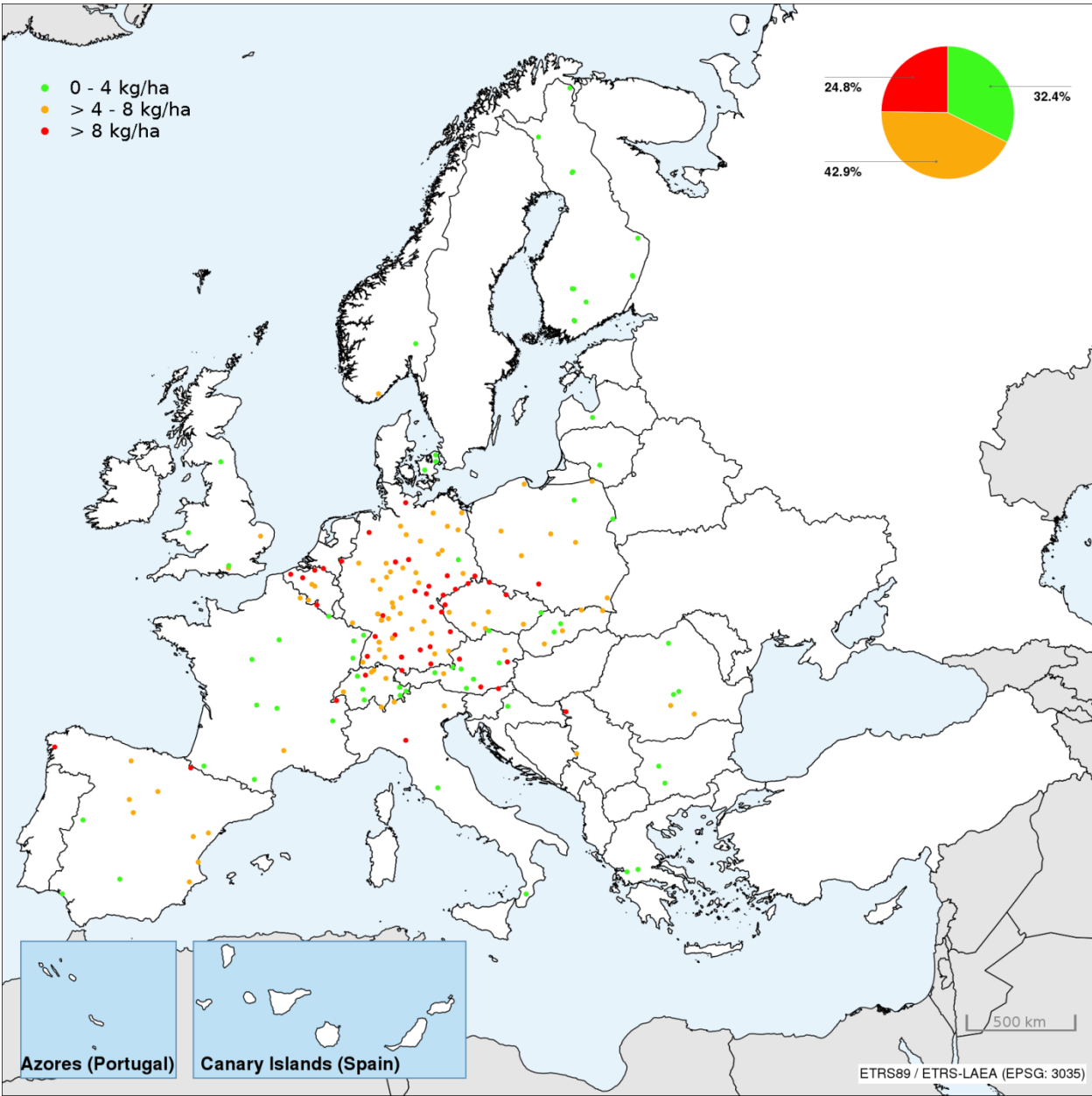
Figure 4-4. Throughfall atmospheric deposition of ammonium nitrogen (NH 4 -N) in European forests in 2014.
