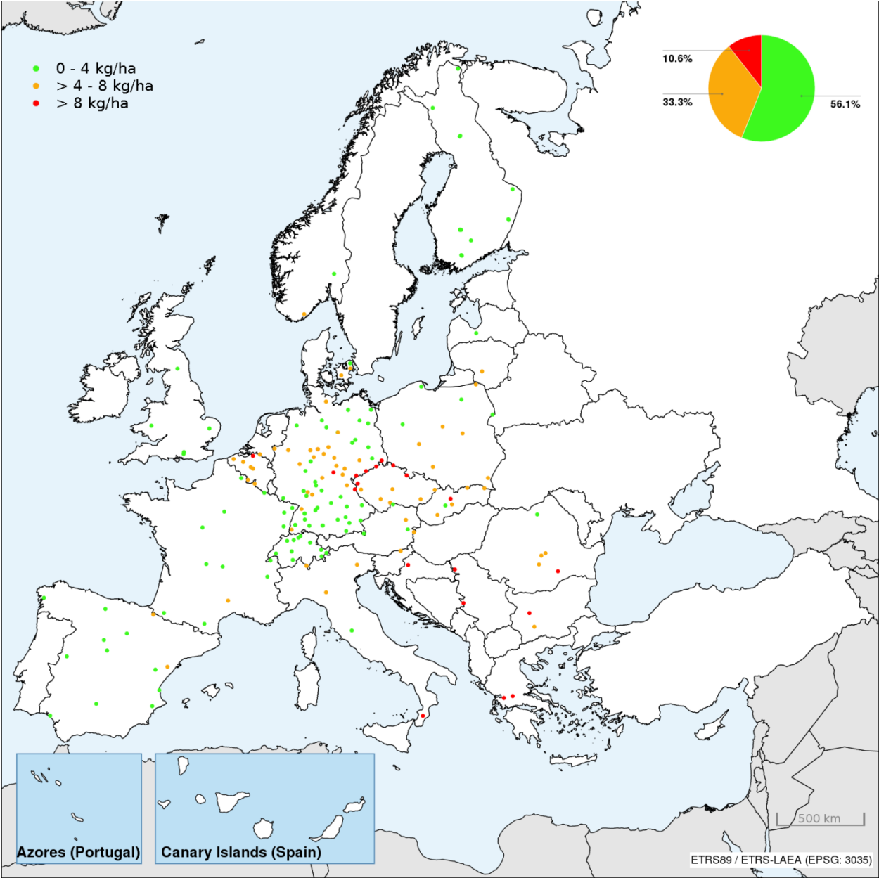
Figure 4-6. Sea-salt corrected throughfall atmospheric deposition of sulphate sulphur ( \text{SO}_4\text{-S} ) in European forests in 2014.
