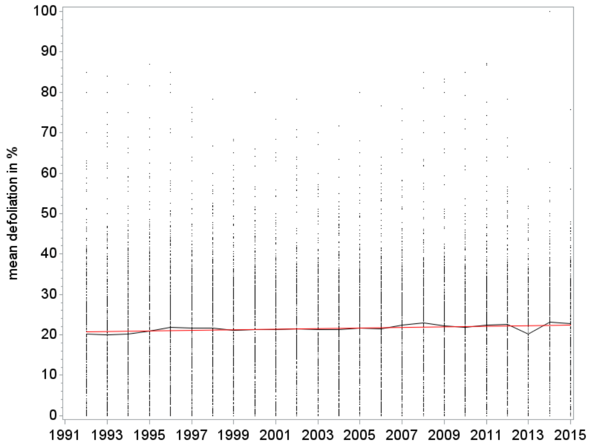
Figure 3-7. Over-all trend (regional Sen's slope = 0.076, p < 0.001 ; minimum length of time span: 20 years, red line) and yearly over-all mean defoliation (black line) of Norway spruce at Level I sites; points represent annual plot means, for clarity these are not interconnected from year to year.
