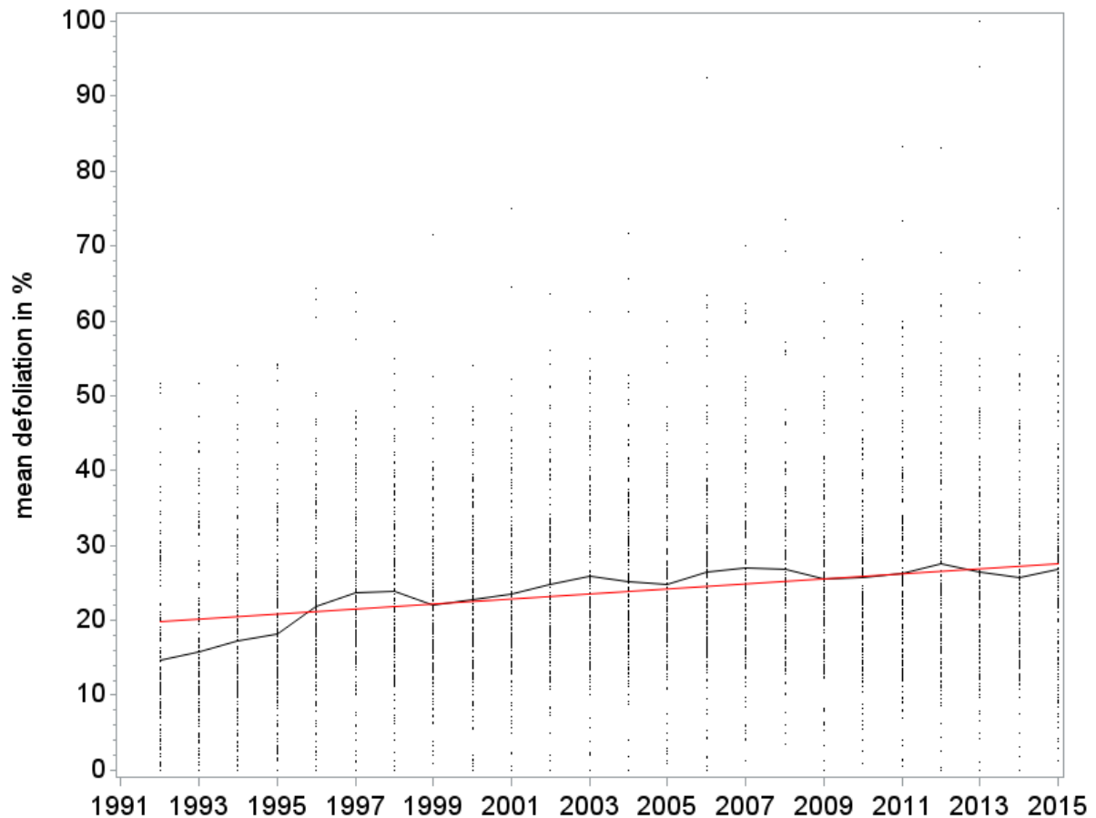
Figure 3-17. Over-all trend (regional Sen's slope = 0.333, p < 0.001 ; minimum length of time span: 20 years, red line) and yearly over-all mean defoliation (black line) of deciduous (sub-) Mediterranean oaks ( Quercus cerris , Q. frainetto , Q. pubescens , Q. pyrenaica ) at Level I sites; points represent annual plot means, for clarity these are not interconnected from year to year.
