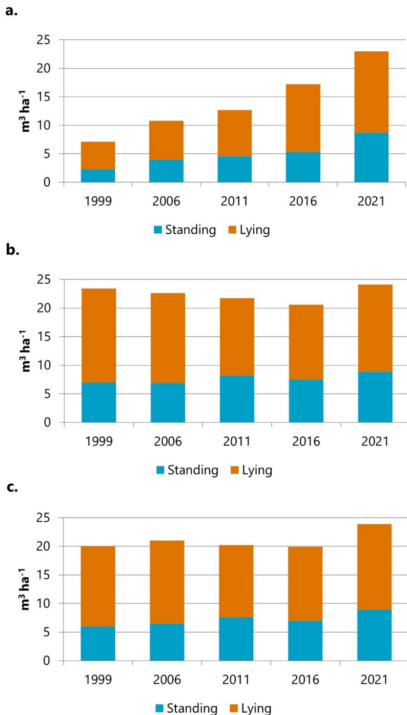
Fig. 21. Mean volume of lying and standing dead wood in productive forests not available for wood supply (FNAWS) according to NFI9–NFI13 in a) South Finland, b) North Finland and c) whole Finland.
