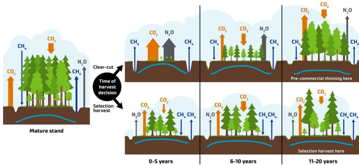
Figure 1. The height of the groundwater level and the emissions and sinks of greenhouse gases, i.e. carbon dioxide ( \text{CO}_2 ), methane ( \text{CH}_4 ) and nitrous oxide ( \text{N}_2\text{O} ) in drained nutrient-rich spruce peatlands of different ages after clear felling and selection harvesting.
