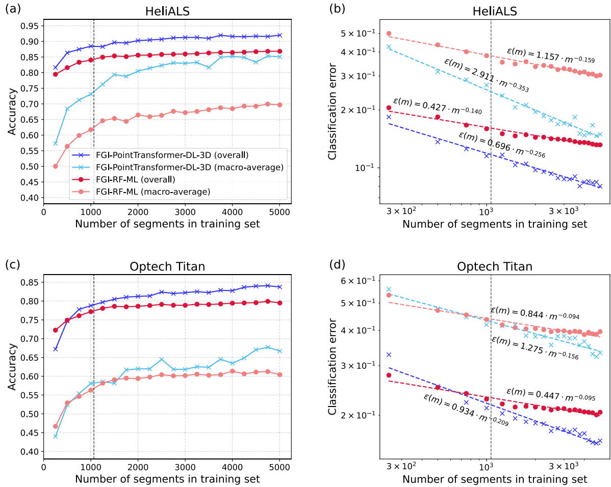
Fig. 9. (a) Overall accuracy (dark color) and macro-average accuracy (light color) of FGI-PointTransformer-DL-3D (blue) and FGI-RF-ML (red) as a function of the number of training segments for HeliALS data. (b) Classification error corresponding to (a) as a function of training set size in logarithmic scale, together with power law fits given by Eq. (7). (c) Same as (a) but using the Optech Titan dataset. (d) Same as (b) but using the Optech Titan dataset. In all panels, the gray vertical lines denote the size of the training set in the benchmark competition. For the DL method, the training set was further divided into training and validation sets for hyperparameter tuning. (For interpretation of the references to color in this figure legend, the reader is referred to the web version of this article.)
