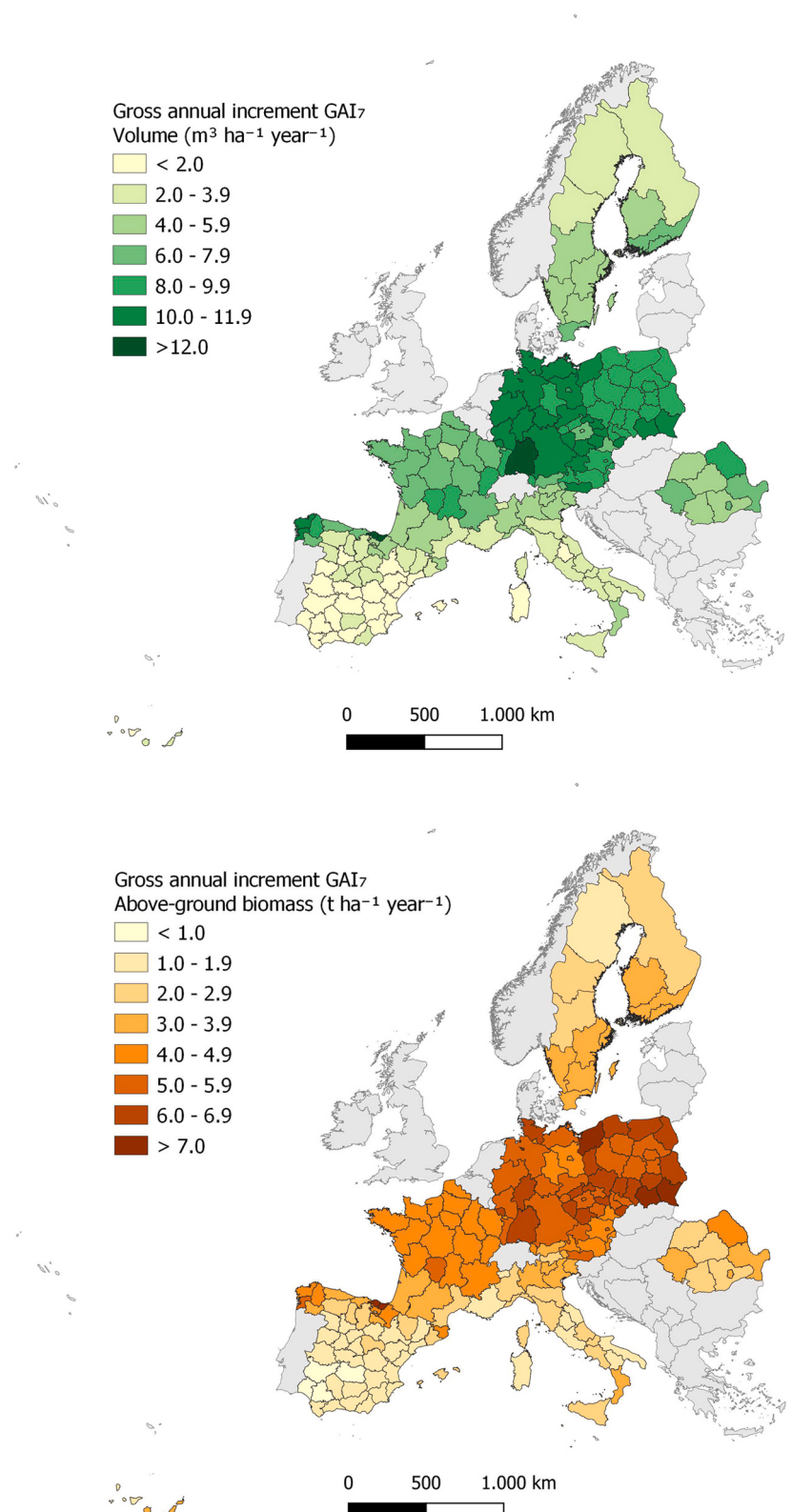
Fig. 4. Harmonised estimates of GAI 7 volume (above) and AGB (below) per ha forest in the NUTS regions of the participating countries. NUTS according to Eurostat (2021).
