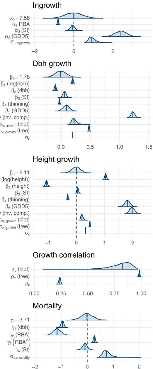
Fig. 2. Posterior distributions of the parameters of the ingrowth sub-model (Eq. (3)), stem diameter (dbh) and height growth sub-model (Eqs. (5)–(6)) and mortality model component (Eq. (11)). The solid vertical lines in the densities denote the posterior means. The names in brackets after the parameters refer to the respective variables.
