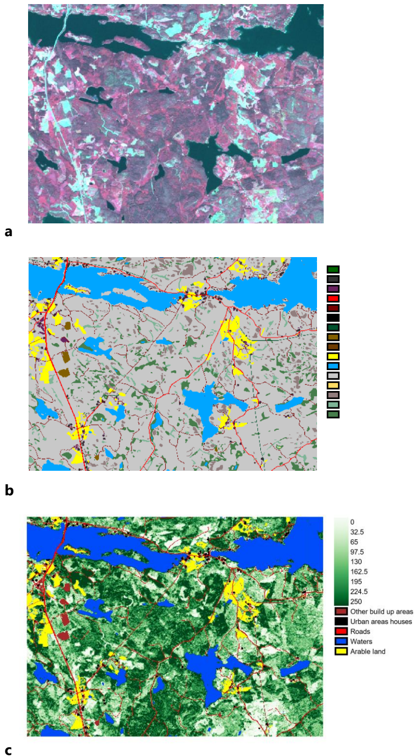
Figure 9. Examples of the Sentinel-2A MSI satellite image, multichannel colour composition of channels 2, 3, and 4 (a); the elements of the topographic map database (b); and MS-NFI-2019 map of total volume (m 3 /ha) with other land use map data (c). Digital map data: contains data from the National Land Survey of Finland topographic database 1/2020.
