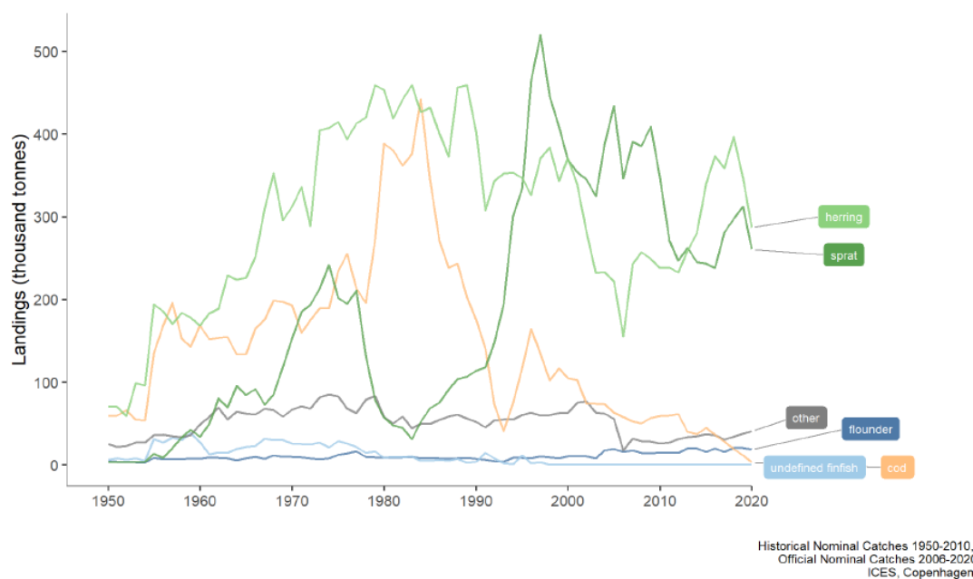
Figure 3.2 Landings (thousand tonnes) from the Baltic Sea in 1950–2020, by species. The five species with the highest landings are displayed separately; the remaining species are aggregated and labelled as “other”. The “undefined finfish” category is due to inadequate reporting in early years. (Source: ICES 2022d).
