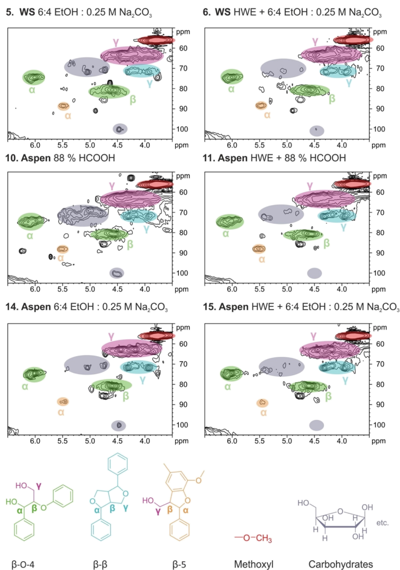
Figure 1. Changes in the lignin phenylpropyl side-chain region with and without HWE treated in mild organosolv conditions (5–6, wheat straw) and (14–15, aspen), and in formic acid conditions (10–11 aspen). Carbohydrate signals were weakened with HWE pretreatment.
