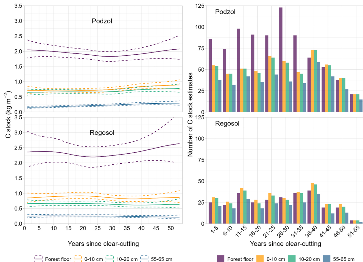
Fig. 4. Soil C stock development after clear-cutting in Pinus dominated stands on Podzol (top-left) and Regosol (bottom-left) soil types. On the right side, number of post clear-cutting soil C stock estimates available for the two taxonomical soil orders, per sample depth interval and post clear-cutting year, binned in 5-year intervals. Solid lines are mean estimates, and dashed lines are 90 % credible intervals.
