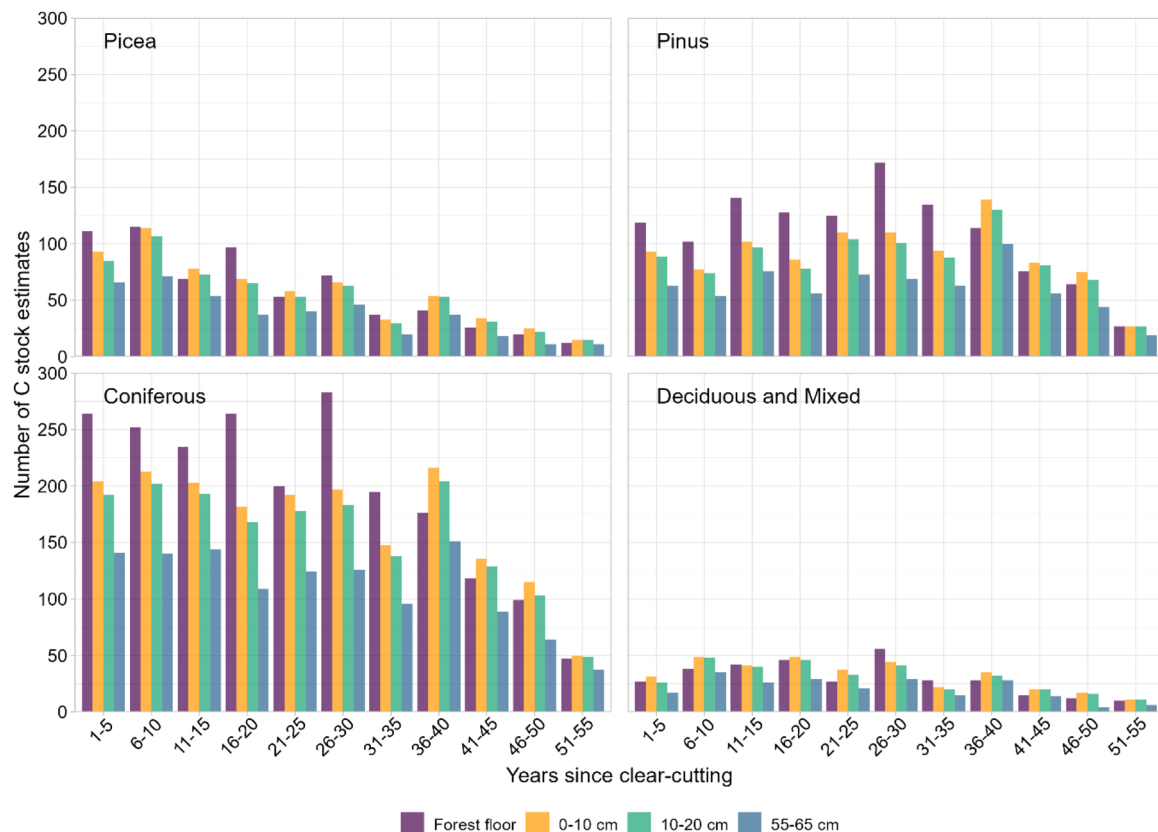
Fig. 3. Number of post clear-cutting C stock estimates available for the different forest categories, per sample depth interval and post clear-cutting year, binned in 5-year intervals.
