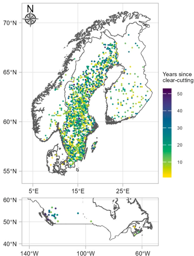
Fig. 1. Geographical distribution of available clear-cut plots in the National Forest Soil Inventories in the Nordics (top) and southern Canada (bottom). Color indicates years passed between clear-cutting and soil sampling.
