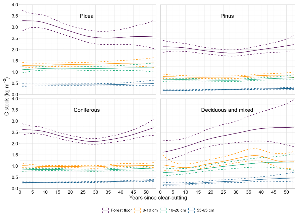
Fig. 2. Post clear-cutting carbon (C) stock development in forest floors and three different mineral soil depth intervals in forest stands dominated by Picea and Pinus tree species (top left and top right, respectively), all coniferous -dominated stands (bottom left), and in deciduous -dominated stands or mixed tree species stands (pooled; bottom right). Solid lines are mean estimates, and dashed lines are 90 % credible intervals.
