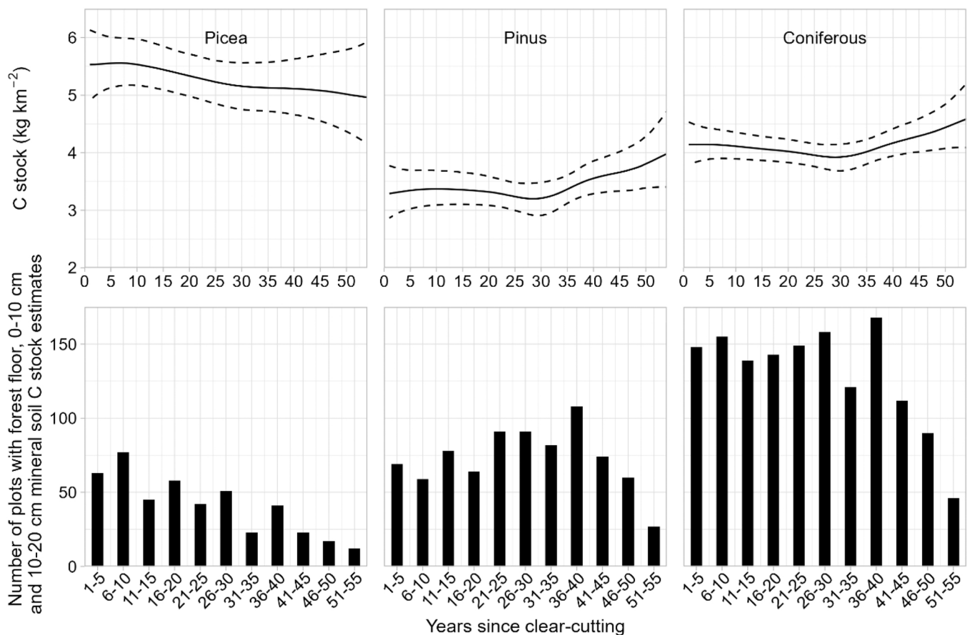
Fig. 5. C stock development in topsoil (forest floor + 0–20 cm mineral soil; top panels) in Picea and Pinus dominated stands and pooled for all coniferous dominated stands. Solid lines are mean estimates, and dashed lines are 90 % credible intervals. Bottom panels show number of plots where C stock estimates were available from all three soil layers (forest floor, 0–10 cm and 10–20 cm mineral soil) along the clear-cutting gradient for each of the forest categories.
