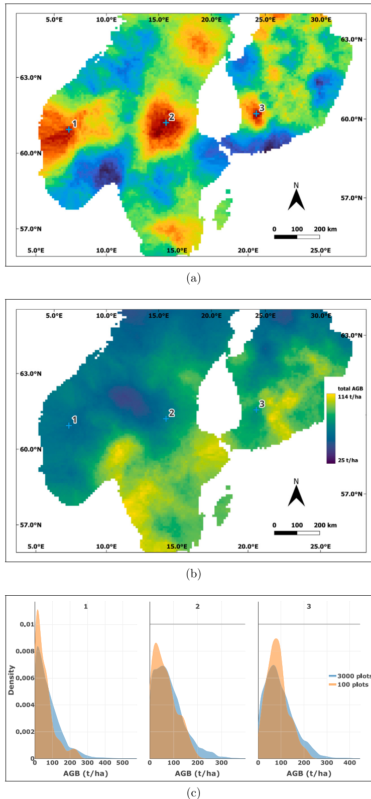
Fig. 8. Map indicating high %bias hotspots (method: RF, R \approx 78 km, and N = 3000 ) (a), hotspot locations over map of observed total AGB (b), and distributions of observed total AGB for each hotspot using the nearest 100 and 3000 sample plots (c).
