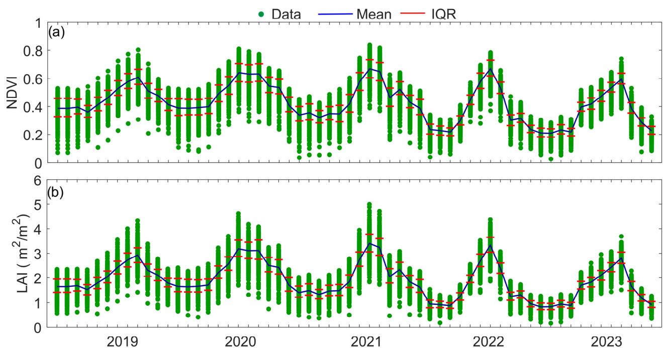
Figure 3. Daily average NDVI and LAI ( \text{m}^2/\text{m}^2 ). (a) Monthly average NDVI from 2019 to 2023, showing seasonal variations in vegetation greenness condition. (b) Monthly average LAI from 2019 to 2023, illustrating changes in forest canopy structure. Green circles represent simulated data, the blue line shows the monthly mean, and the red lines indicate the interquartile range (IQR, Q3–Q1), representing the middle 50% of the data.
