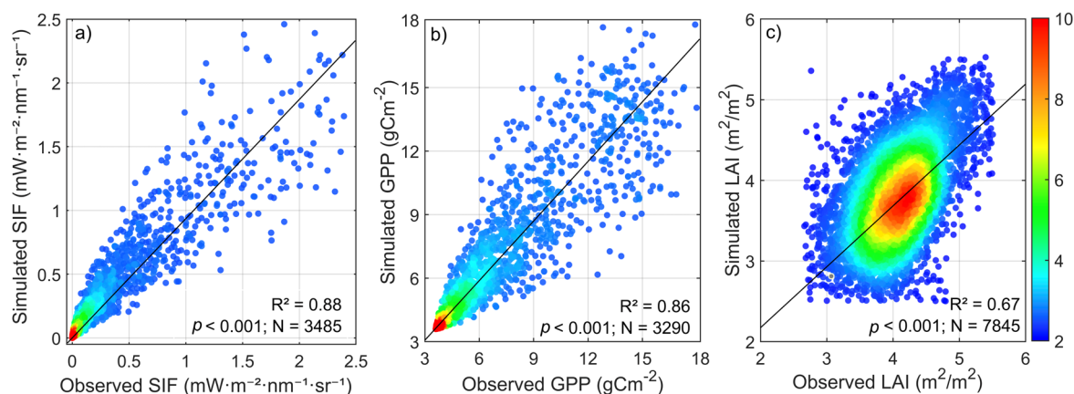
Figure 8. Relationship between modeled and observed values of (a) SIF, (b) GPP, and (c) LAI. The figure illustrates the agreement between model simulations and observations, showing the model's accuracy in measured chlorophyll fluorescence, photosynthetic activity, and mangrove leaf area dynamics. The color gradient from cold blue to warm red indicates the density of individual data points, ranging from 2 to 10.
