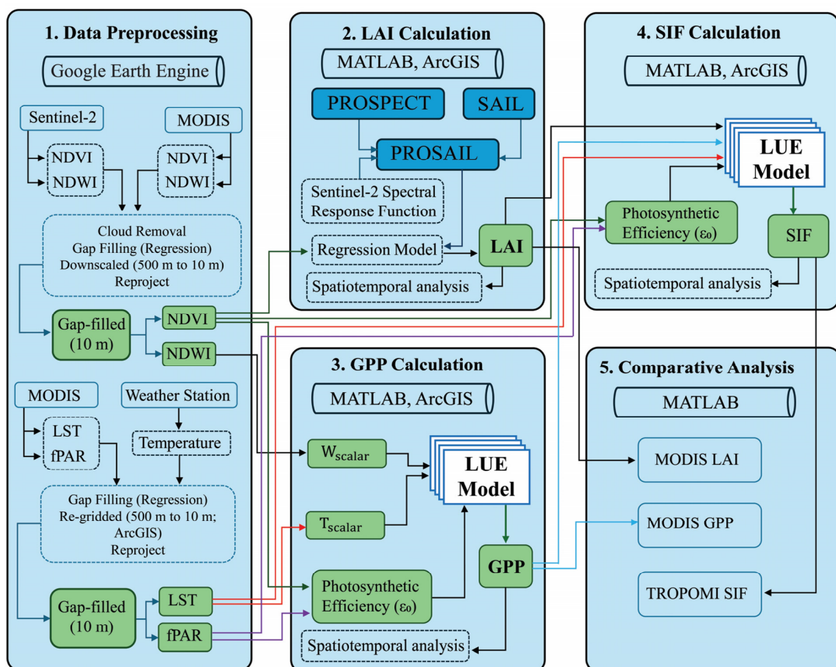
Figure 2. Workflow for estimating Leaf Area Index (LAI), Gross Primary Productivity (GPP), and Solar-Induced Chlorophyll Fluorescence (SIF). Sentinel-2, MODIS, TROPOMI, and weather station data were processed in Google Earth Engine and ArcGIS (version: 3.2) to generate vegetation indices, remove clouds, and downscale resolution. LAI was retrieved using the PROSAIL radiative transfer model, GPP was estimated with a Light Use Efficiency (LUE) model, and SIF was derived through an LUE-based framework. Analyses conducted in Google Earth Engine, MATLAB (version: 24.2), and ArcGIS (version: 3.2) were validated against independent MODIS and TROPOMI datasets.
