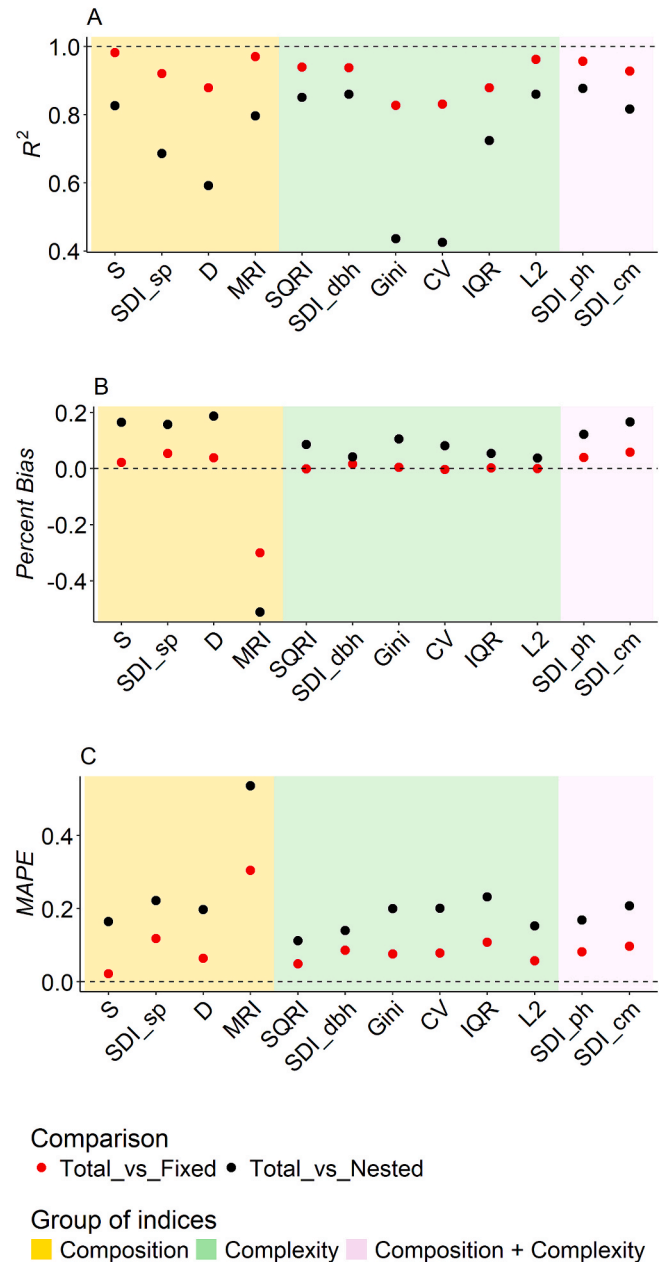
Fig. 3. Metrics evaluating the performance of the structural indices benchmarking the Total against Fixed and Nested plot designs for Spain. Refer to Table 2 for a detailed description of the indices. Perc_bias = Percentage of bias, MAPE = Mean absolute percentage error. In the R^2 panel (A), the horizontal dashed line at 1 denotes the maximum achievable R^2 score while the zero line in the Perc_bias and MAPE plots (B and C) acts as a reference point.
