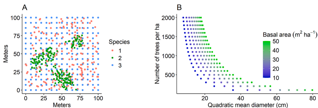
Fig. 1. A: Representation of a 1 ha plot with three species and a basal area equal to 25 m 2 ha -1 and a tree density of 600 trees per ha. Species 1 (red dots) follows a random spatial pattern, Species 2 (green dots) a clustered pattern and Species 3 (blue dots) a regular pattern. B: Relationship between number of trees per ha, quadratic mean diameter and basal area for the whole array of simulated plots. (For interpretation of the references to colour in this figure legend, the reader is referred to the web version of this article.)
