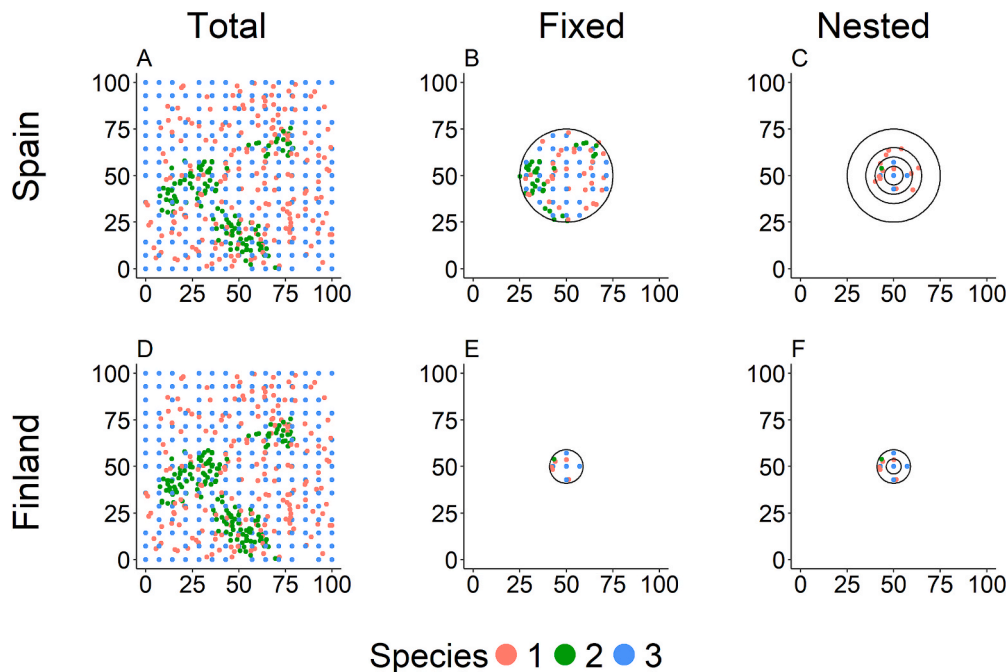
Fig. 2. Representation of a Total (basal area equal to 25 m 2 ha -1 and a tree density of 600 trees per ha), Fixed and Nested plot for Spain and Finland in a three-species plot. Units on the axes refer to meters. Species 1 (red dots) follows a random spatial pattern, Species 2 (green dots) a clustered pattern and Species 3 (blue dots) a regular pattern. (For interpretation of the references to colour in this figure legend, the reader is referred to the web version of this article.)
