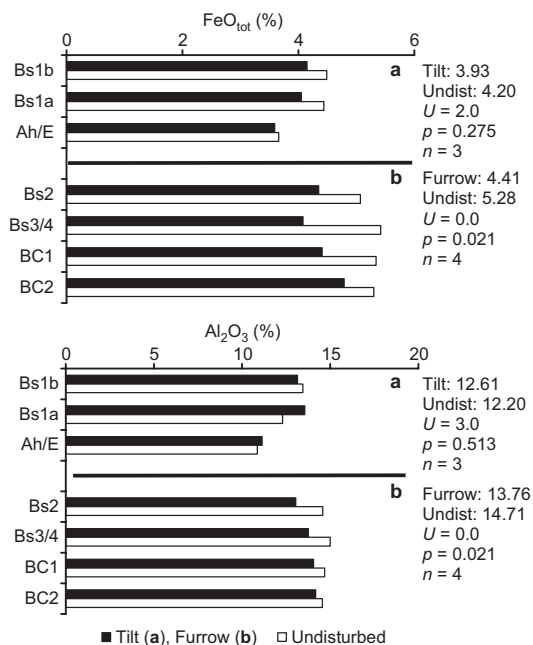
Fig. 6. FeO tot (total iron) and Al 2 O 3 concentrations (% d.w.) in the Bs and Ah/E horizons in (a) the tilt and (b) the Bs and BC horizons in the furrow. For comparison, the concentrations in the corresponding undisturbed soil horizons (undisturbed in non-ploughed area) for the tilt and furrow horizons are also shown. Mean values for the whole tilt part of the soil containing the three soil layers and for the corresponding undisturbed soil layers are given before the test (Mann-Whitney U -test) results next to the panels. For further explanations see Figs. 1 and 3.
