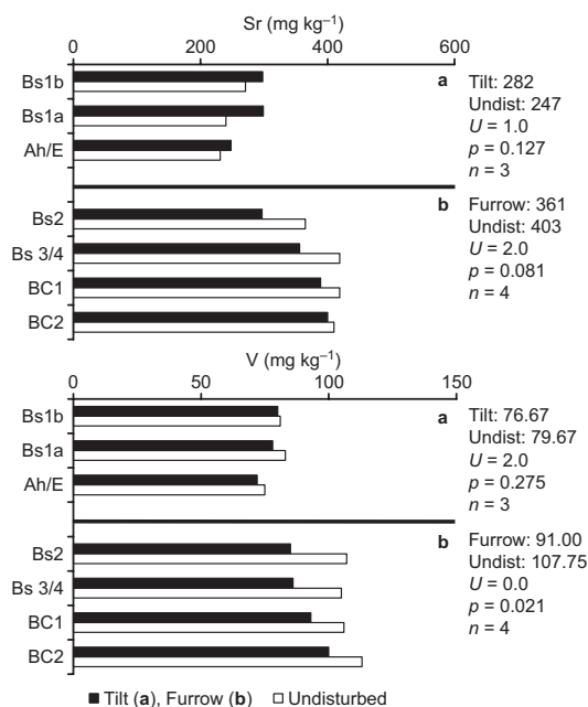
Fig. 4. Sr and V concentrations (mg kg -1 d.w.) in the Bs and Ah/E horizons in (a) the tilt and (b) the Bs and BC horizons in the furrow. For comparison, the concentrations in the corresponding undisturbed soil horizons (undisturbed in non-ploughed area) for the tilt and furrow horizons are also shown. Mean values for the whole tilt part of the soil containing the three soil layers and for the corresponding undisturbed soil layers are given before the test (Mann-Whitney U -test) results next to the panels. For further explanations see Figs. 1 and 3.
