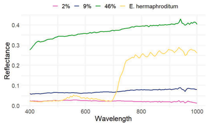
Fig. 4. Hyperspectral reflectance spectra at calibration panels (2–46%) and a typical E.-hermaphroditum -dominated spot in the scene. Spectra were obtained by weighted averaging over small ( < 0.2\text{m}^2 ) hand-drawn areas at selected locations.
