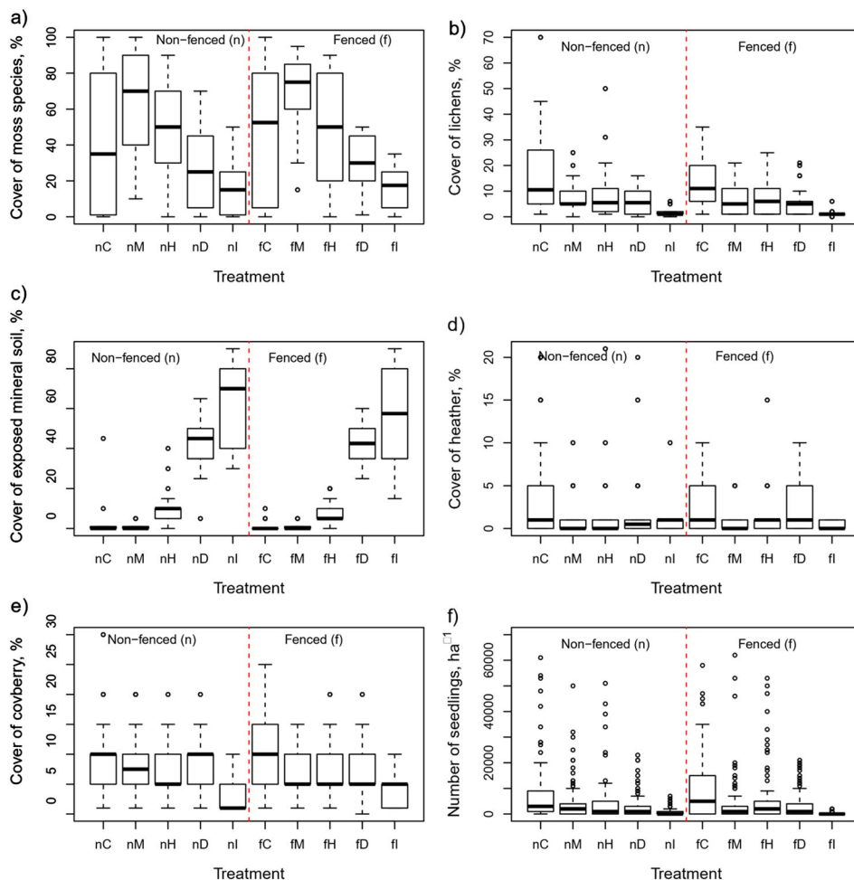
Figure A1.1. Raw distributions of moss species cover (a), lichen cover (b), exposed mineral soil (c), heather cover (d), cowberry cover (e) and the number of seedlings per ha by the treatments consisting of soil fencing and soil treatment. Abbreviations for the treatments: n denotes non-fenced, and f fenced, C denotes control, M denotes logging machine, H denotes Huminmix, D denotes disk trenching and I intensive soil scarification (> 50% exposed mineral soil). The distributions have been computed based on the circle plots ( n = 300 ).
