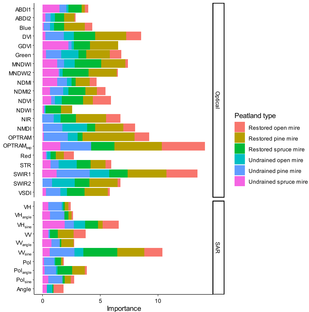
Fig. 5. Variable importance for the models with explanatory variables calculated from multi-sensor data (combination of optical and C-band SAR data). The boxes represent summed variable importance over all sites. Variable names are explained in Table 2.
