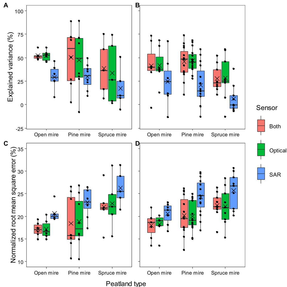
Fig. 4. The % of explained variance (A, B) and normalized root mean square error (C, D) boxplots for undrained (A, C) and restored (B, D) peatland sites. Separate boxplots are shown for models having variables from both sensor types, optical data, and C-band SAR data, as well as for the three peatland habitat types. Median value is shown with the center line, and first and third quartiles with lower and upper hinges, respectively. Whiskers extend no further than 1.5 times the interquartile range from the hinge. Each dot in the boxplot is the statistic value for one peatland site while mean value for a boxplot is shown with “x”.
