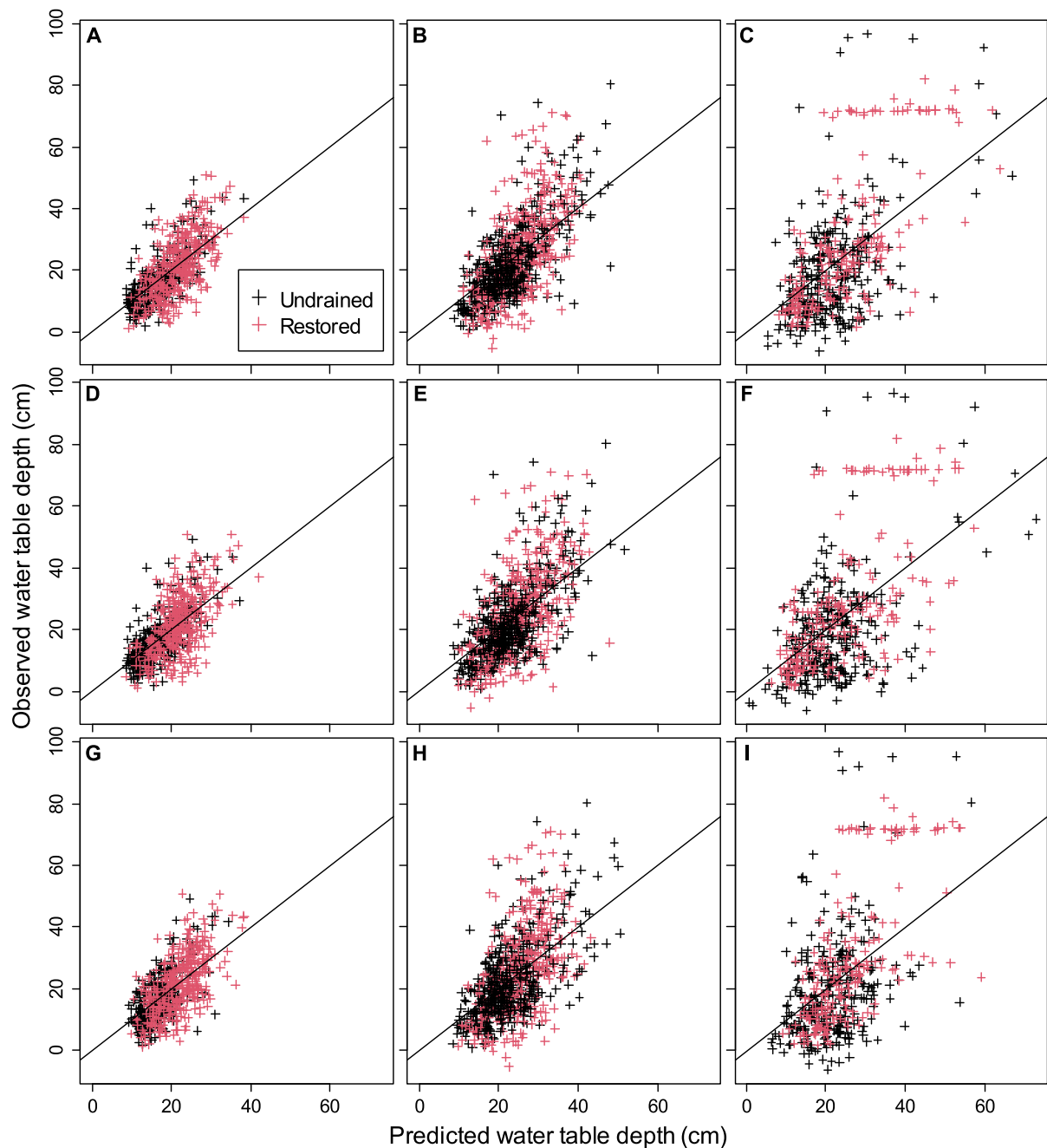
Fig. 3. Observed (y-axis) and predicted (x-axis) water table depths for open mire (A, D, G), pine mire (B, E, H), and spruce mire (C, F, I) models with multi-sensor data (A-C), optical data (D-F), and C-band SAR data (G-I). Black line is 1:1 line. Predicted values are based on the models which included data from several sites and were trained separately for the different habitat types and management options. Model performance results are presented in Table 3. Note that observations and predictions for undrained (black symbols) and drained peatland sites (red symbols) are drawn in the same figures.
