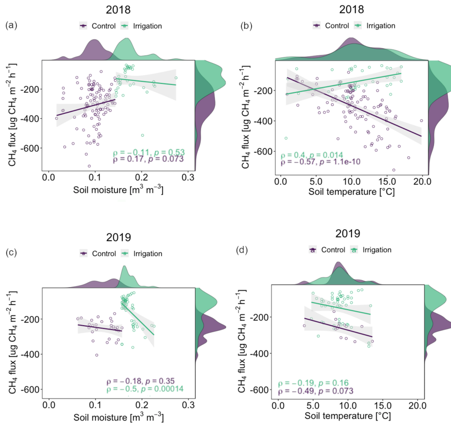
Figure 8. Correlations (Pearson's coefficient, \rho ) between soil moisture and CH 4 flux ( a, c ) and soil temperature and CH 4 flux ( b, d ) with smoothed frequency histograms in 2018 and 2019. The emission case of 27 June 2019 was removed from the data in the correlation analyses for more clear presentation.
