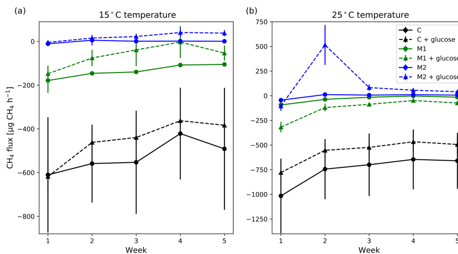
Figure 9. Weekly mean CH 4 flux measured at 15 °C ( a ) and 25 °C ( b ) without (solid lines) and with (dashed lines) added glucose on different moisture levels (black: control; green: low added moisture; blue: high added moisture). The error bars show the standard error of the mean ( n = 3 ). Positive flux values indicate net emission and negative values indicate net uptake.
