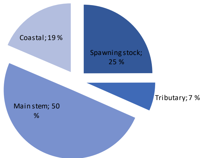
Figure 51. The total amount of salmon belonging to Anárjohka/Inarijoki in 2016-2019, distributed into surviving spawning stock and salmon caught in fisheries in either coastal, main stem or Anárjohka/Inarijoki fisheries. The percentages in the figure represent the proportion of the pre-fishery abundance that survives to spawning or are caught in coastal, main stem or tributary fisheries.
