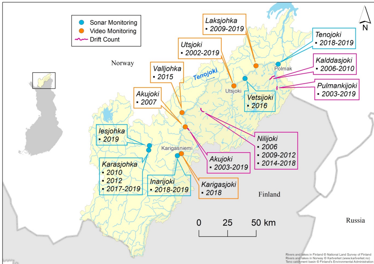
Figure 8. Map of the Tana/Teno river system indicating the most important adult salmon counting sites and counting methods between 2002 and 2019.
