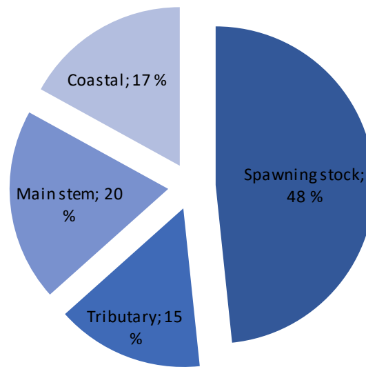
Figure 33. The total amount of salmon belonging to Ohcejohka/Utsjoki in 2016-2019, distributed into surviving spawning stock and salmon caught in fisheries in either coastal, main stem or Ohcejohka/Utsjoki fisheries. The percentages in the figure represent the proportion of the pre-fishery abundance that survives to spawning or are caught in coastal, main stem or tributary fisheries.
