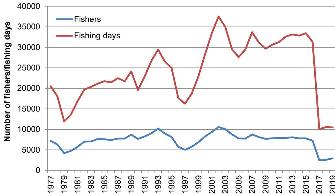
Figure 4. Number of tourist fishers (blue) and daily fishing licences (red) in the Tana/Teno river system on the Finnish side in 1977-2019.
