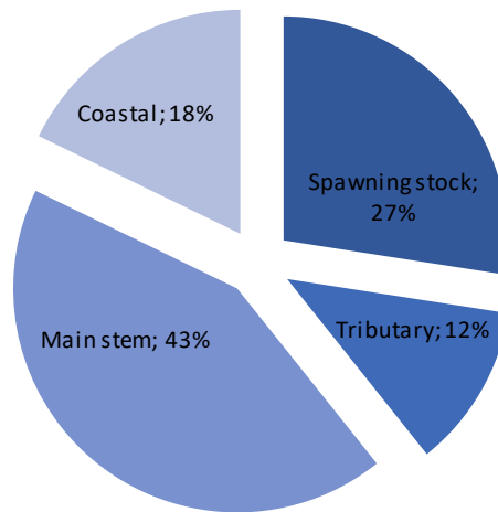
Figure 47. The total amount of salmon belonging to Kárášjohka in 2016-2019, distributed into surviving spawning stock and salmon caught in fisheries in either coastal, main stem or Kárášjohka fisheries. The percentages in the figure represent the proportion of the pre-fishery abundance that survives to spawning or are caught in coastal, main stem or tributary fisheries.
