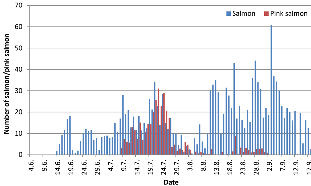
Figure 18. Estimated numbers of salmon (1 593) and pink salmon (353) in the Anárjohka/Inarijoki sonar count in 2019. Separation of salmon and pink salmon is based on length distribution data of sonar count and video monitoring data from the sonar counting line.
