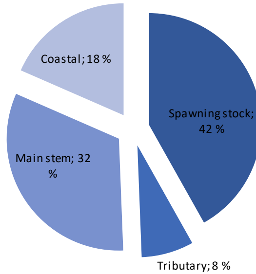
Figure 31. The total amount of salmon belonging to Veahčajohka/Vetsijoki in 2016-2019, distributed into surviving spawning stock and salmon caught in fisheries in either coastal, main stem or Veahčajohka/Vetsijoki fisheries. The percentages in the figure represent the proportion of the pre-fishery abundance that survives to spawning or are caught in coastal, main stem or tributary fisheries.
