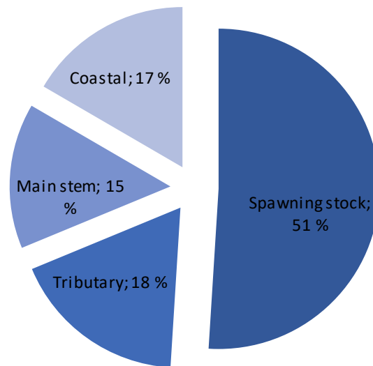
Figure 25. The total amount of salmon belonging to Máskejohka in 2016-2019, distributed into surviving spawning stock and salmon caught in fisheries in either coastal, main stem or Máskejohka fisheries. The percentages in the figure represent the proportion of the pre-fishery abundance that survives to spawning or are caught in coastal, main stem or tributary fisheries.
