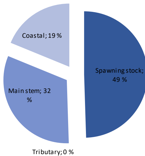
Figure 37. The total amount of salmon belonging to Leavvajohka in 2016-2019, distributed into surviving spawning stock and salmon caught in fisheries in either coastal, main stem or Leavvajohka fisheries. The percentages in the figure represent the proportion of the pre-fishery abundance that survives to spawning or are caught in coastal, main stem or tributary fisheries.
