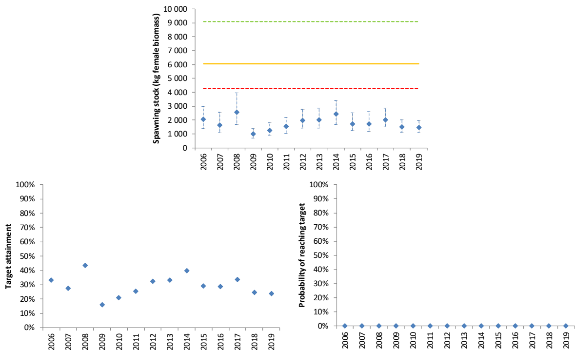
Figure 48. The estimated spawning stock (top row), percent truncated spawning target attainment (bottom row, left) and probability of reaching the spawning target (bottom row, right) in the period 2006-2019 in the Norwegian tributary Iešjohka.
