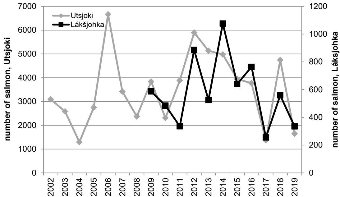
Figure 9. Video counts of ascending adult salmon at the video monitoring sites in the Ohcejohka/Utsjoki and Láksjohka in 2002-2019. Sea age groups are combined. Note: the data in 2017 is not fully comparable to other years because of challenging environmental conditions affecting the count accuracy in both locations. The Ohcejohka/Utsjoki 2019 adult count is an estimate, as a small fraction of the data is still being analysed when writing this report.
