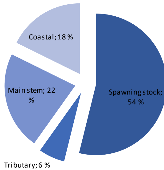
Figure 29. The total amount of salmon belonging to Lákšjohka in 2016-2019, distributed into surviving spawning stock and salmon caught in fisheries in either coastal, main stem or Lákšjohka fisheries. The percentages in the figure represent the proportion of the pre-fishery abundance that survives to spawning or are caught in coastal, main stem or tributary fisheries.
