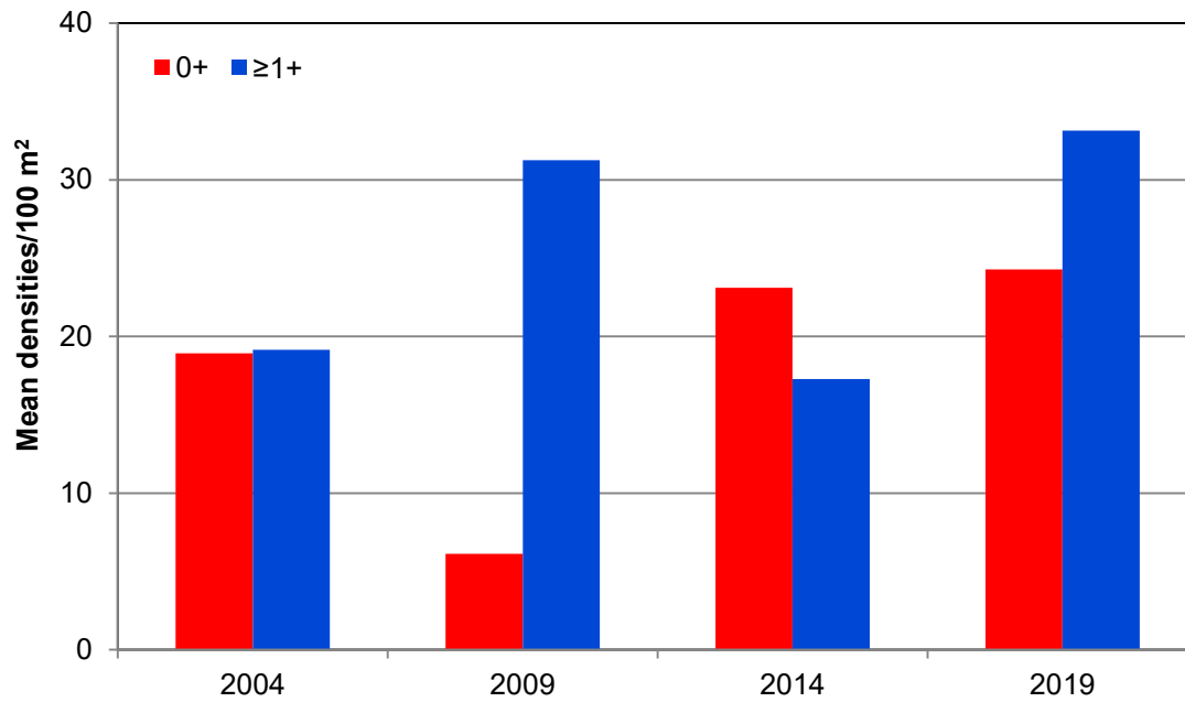
Figure 7. Mean densities (fish/100m 2 ; one pass) of salmon fry (0+) and parr (≥1+) in the River Tsarsjoki in 2004, 2009, 2014 and 2019. The mean densities are based on data from 26 sampling sites (see Figure 6).
