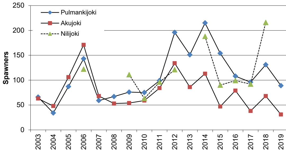
Figure 10. Snorkelling counts of spawning salmon in the rivers Buolbmátjohka/Pulmankijoki, Áhkojohka/Akujoki and Njiljohka/Nilijoki in 2003-2019. Sea-age groups are combined. Njiljohka/Nilijoki was not counted in 2019 because of extremely low water levels during the monitoring period.
