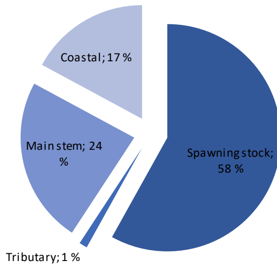
Figure 35. The total amount of salmon belonging to Goahppelašjohka/Kuoppilasjoki in 2016-2019, distributed into surviving spawning stock and salmon caught in fisheries in either coastal, main stem or Goahppelašjohka/Kuoppilasjoki fisheries. The percentages in the figure represent the proportion of the pre-fishery abundance that survives to spawning or are caught in coastal, main stem or tributary fisheries.
