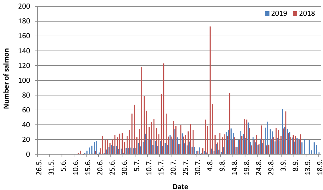
Figure 15. Estimated daily numbers of ascending salmon ( \geq 45 cm) in the Anárjohka/Inarjoki sonar count in 2018 (red bars) and 2019 (blue bars). All size categories are combined. The estimate of the total ascendance through the site in 2018 and 2019 was 2 848 and 1 593 salmon, respectively.
