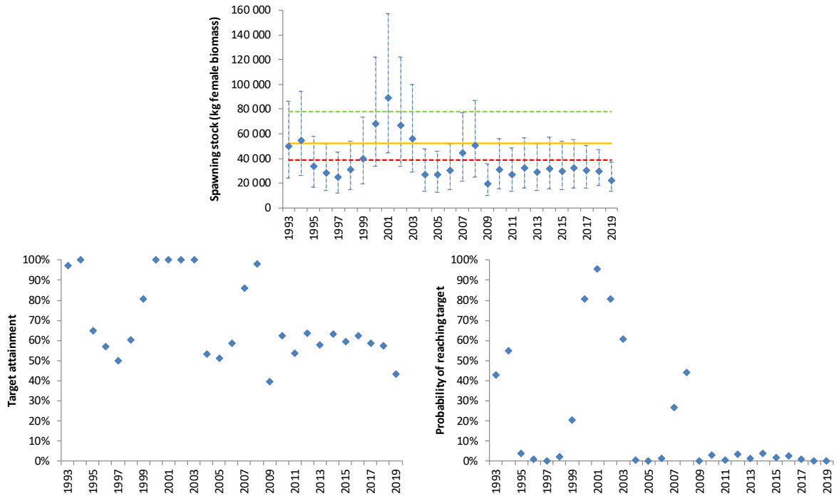
Figure 52. The estimated spawning stock (top row), percent truncated spawning target attainment (bottom row, left) and probability of reaching the spawning target (bottom row, right) in the period 1993-2019 for Tana/Teno (total).
