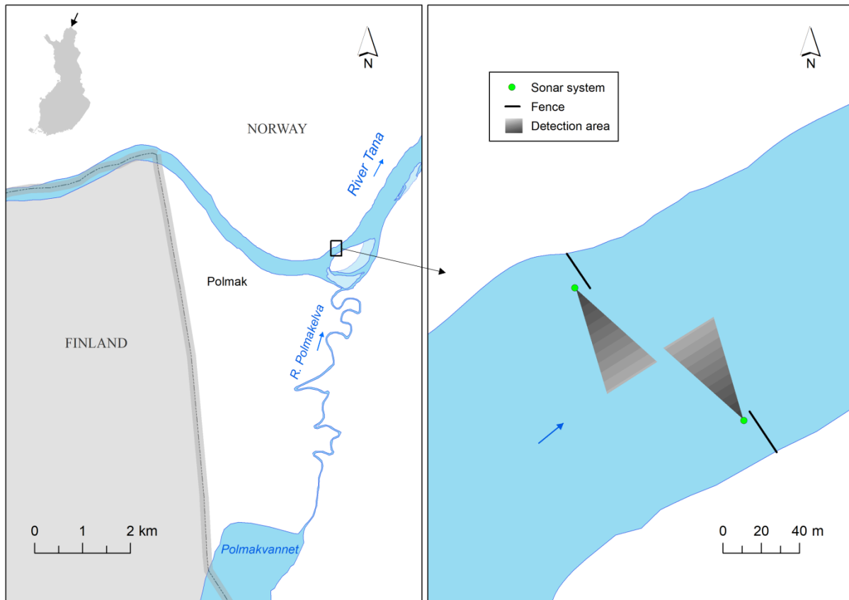
Figure 12. Map of the Tana/Teno main stem sonar counting site including the locations of the two sonar units and guiding fences in 2019.
