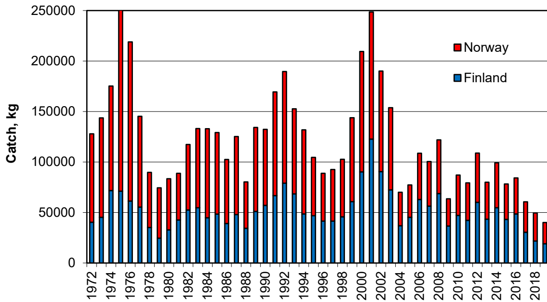
Figure 2. Estimated total salmon catch (kg) in the Tana/Teno river system in Norway and Finland in 1972-2019.
