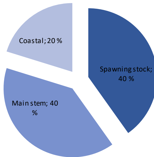
Figure 23. The total amount of salmon belonging to Tana MS in 2016-2019, distributed into surviving spawning stock and salmon caught in fisheries in either coastal or main stem fisheries. The percentages in the figure represent the proportion of the pre-fishery abundance that survives to spawning or are caught in coastal or main stem fisheries.
