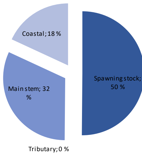
Figure 39. The total amount of salmon belonging to Báišjohka in 2016-2019, distributed into surviving spawning stock and salmon caught in fisheries in either coastal, main stem or Báišjohka fisheries. The percentages in the figure represent the proportion of the pre-fishery abundance that survives to spawning or are caught in coastal, main stem or tributary fisheries.
