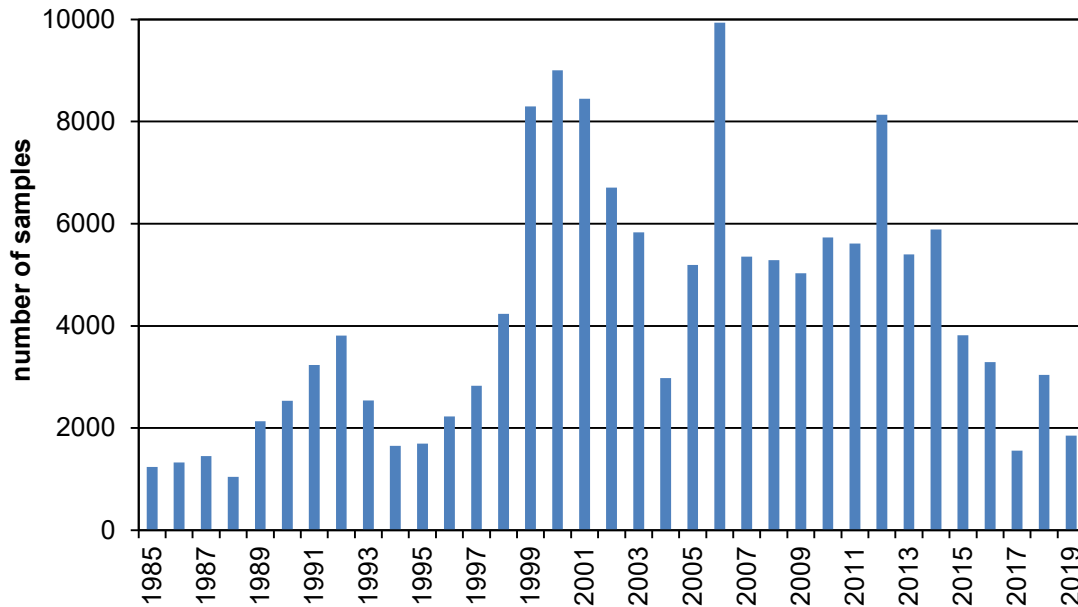
Figure 1. Number of salmon scale samples collected annually from the Tana/Teno system in 1985-2019 including both Finnish and Norwegian samples.
