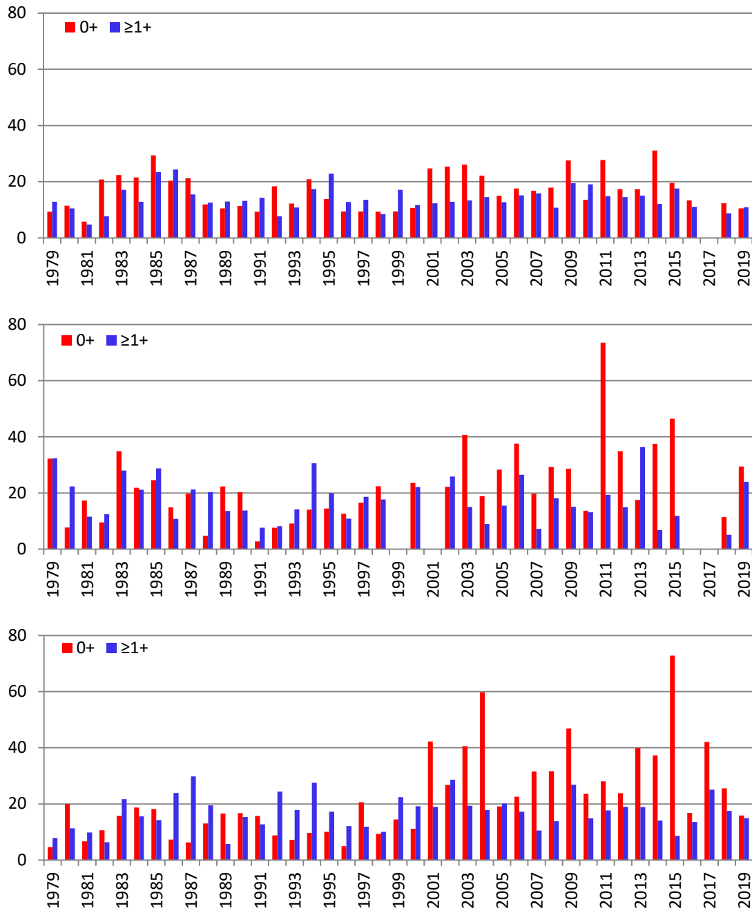
Figure 5. Mean densities (fish/100m 2 ; one pass) of salmon fry (0+) and parr (≥1+) at permanent electrofishing sites in the rivers Tana/Teno, Ohcejohka/Utsjoki and Anárjohka/Inarijoki in the years 1979-2019. Note: this data only includes electrofishing sites (Tana/Teno 17-22 sites, Ohcejohka/Utsjoki 11-12 sites and Anárjohka/Inarijoki 5-7 sites) that have been the same throughout the monitoring period.
