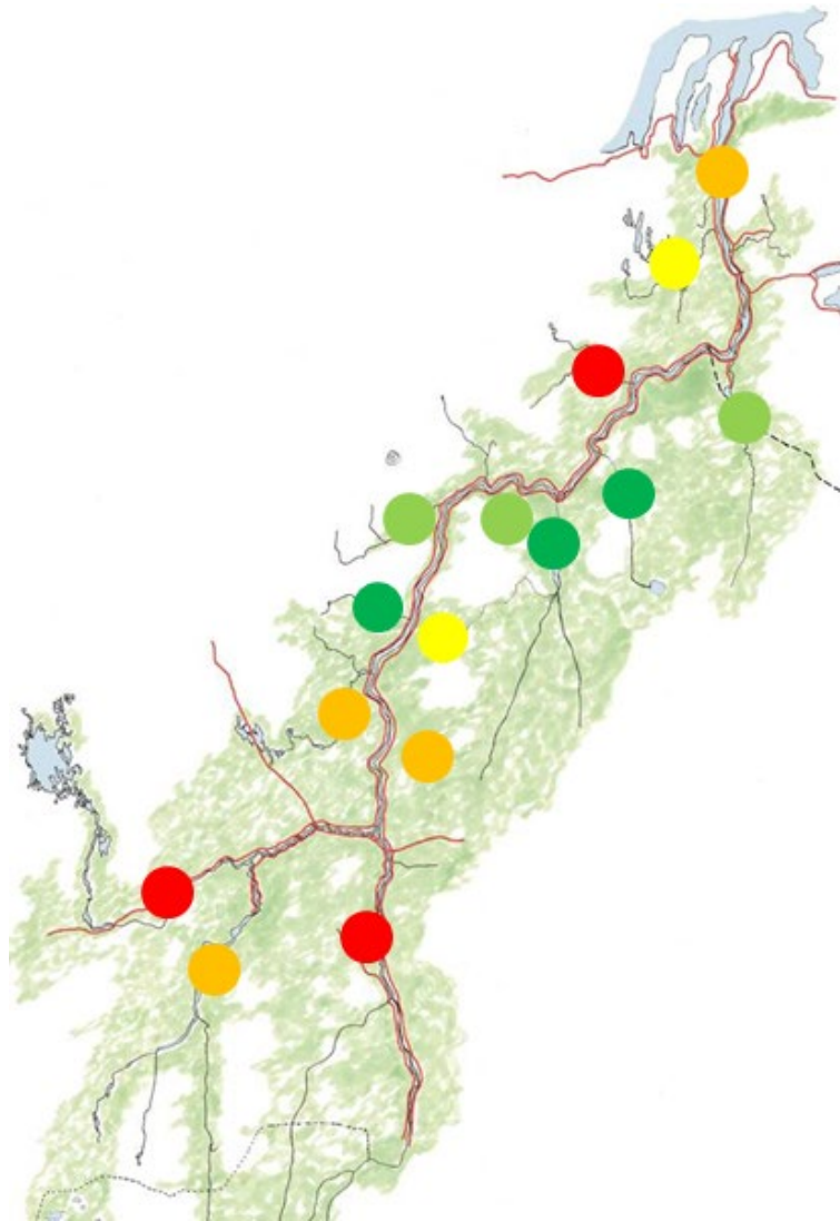
Figure 54. Map summary of the 2016-2019 stock status of the evaluated parts of the Tana/Teno river system. Symbol colour designates stock status over the last four years. Possible colours are: Dark green = overall probability of attaining spawning target higher than 75 %, overall target attainment over 140 %. Light green = overall probability of attaining spawning target higher than 75 %. Yellow = overall probability of attaining spawning target between 40 and 74 %, overall target attainment above 75 %. Orange = overall probability of attaining spawning target below 40 %, stock has had an exploitable surplus in at least 3 of the last 4 years. Red = stock had an exploitable surplus in less than 3 of the last 4 years.
