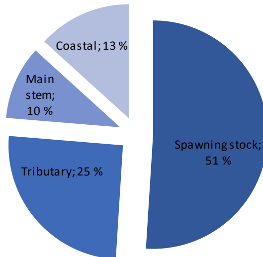
Figure 27. The total amount of salmon belonging to Buolbmátjohka/Pulmankijoki in 2016-2019, distributed into surviving spawning stock and salmon caught in fisheries in either coastal, main stem or Buolbmátjohka/Pulmankijoki fisheries. The percentages in the figure represent the proportion of the pre-fishery abundance that survives to spawning or are caught in coastal, main stem or tributary fisheries.
