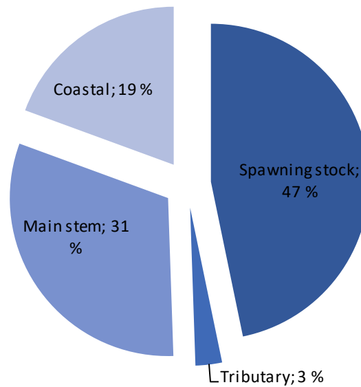
Figure 43. The total amount of salmon belonging to Váljohka in 2016-2019, distributed into surviving spawning stock and salmon caught in fisheries in either coastal, main stem or Váljohka fisheries. The percentages in the figure represent the proportion of the pre-fishery abundance that survives to spawning or are caught in coastal, main stem or tributary fisheries.
