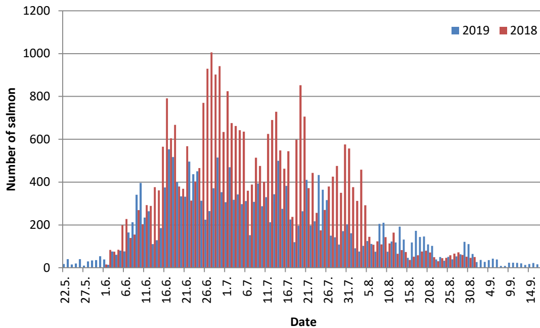
Figure 13. Estimated daily numbers of ascending salmon ( \geq 45 cm) in the Tana/Teno main stem sonar count at Polmak in 2018 (red bars) and 2019 (blue bars). All size categories are combined. The estimate of the total ascendance through the site in 2018 and 2019 was 32 455 and 21 013 salmon, respectively.
