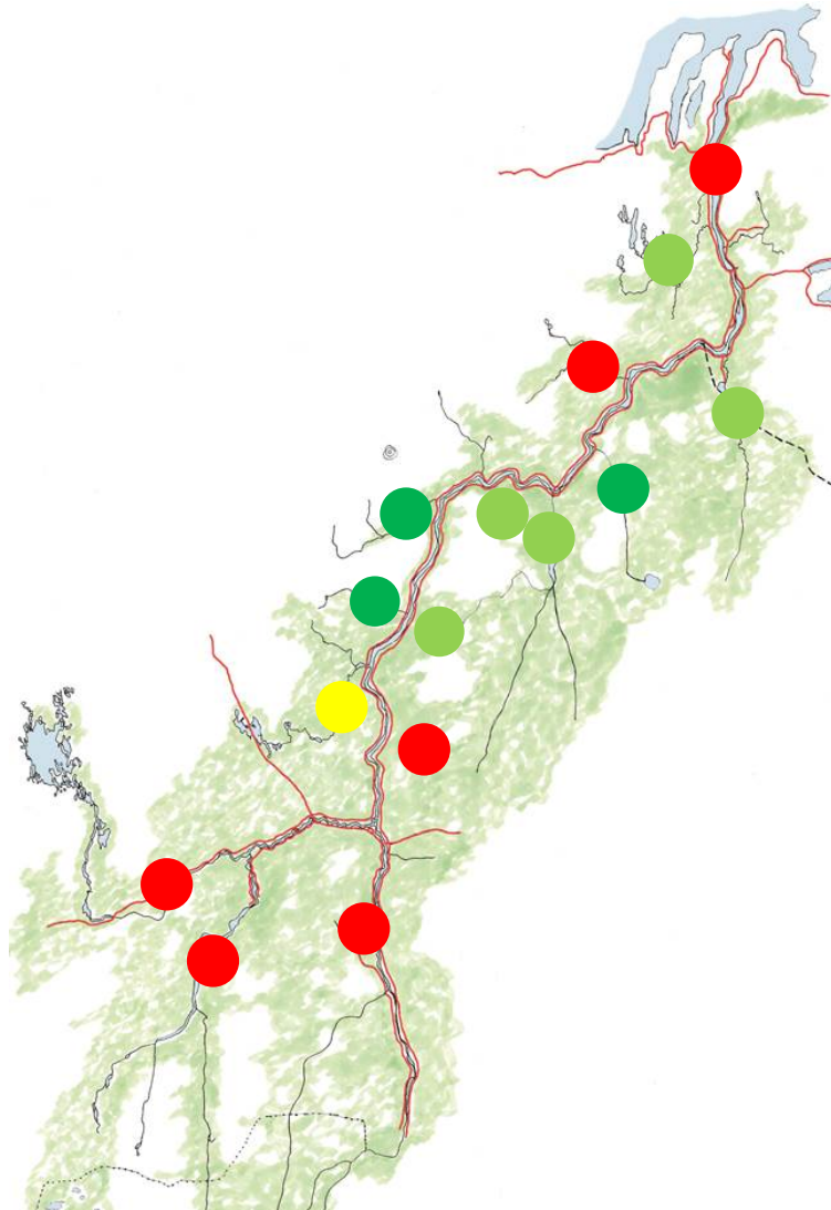
Figure 55. Map summary of the estimated overexploitation experienced in various parts of the Tana/Teno river system in the years 2016-2019. Symbol colour represents the extent of the overexploitation (in terms of percentages of the spawning target). Dark green = no effect (0 % of the spawning target), light green = small effect (<10 %), yellow = moderate effect (10-30 %), red = large effect (>30 %).
