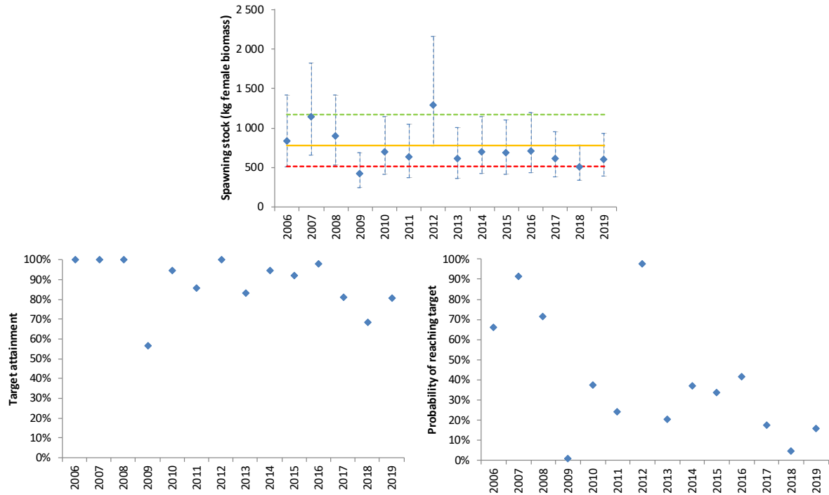
Figure 42. The estimated spawning stock (top row), percent truncated spawning target attainment (bottom row, left) and probability of reaching the spawning target (bottom row, right) in the period 2006-2019 in the Norwegian tributary Våljohka.
