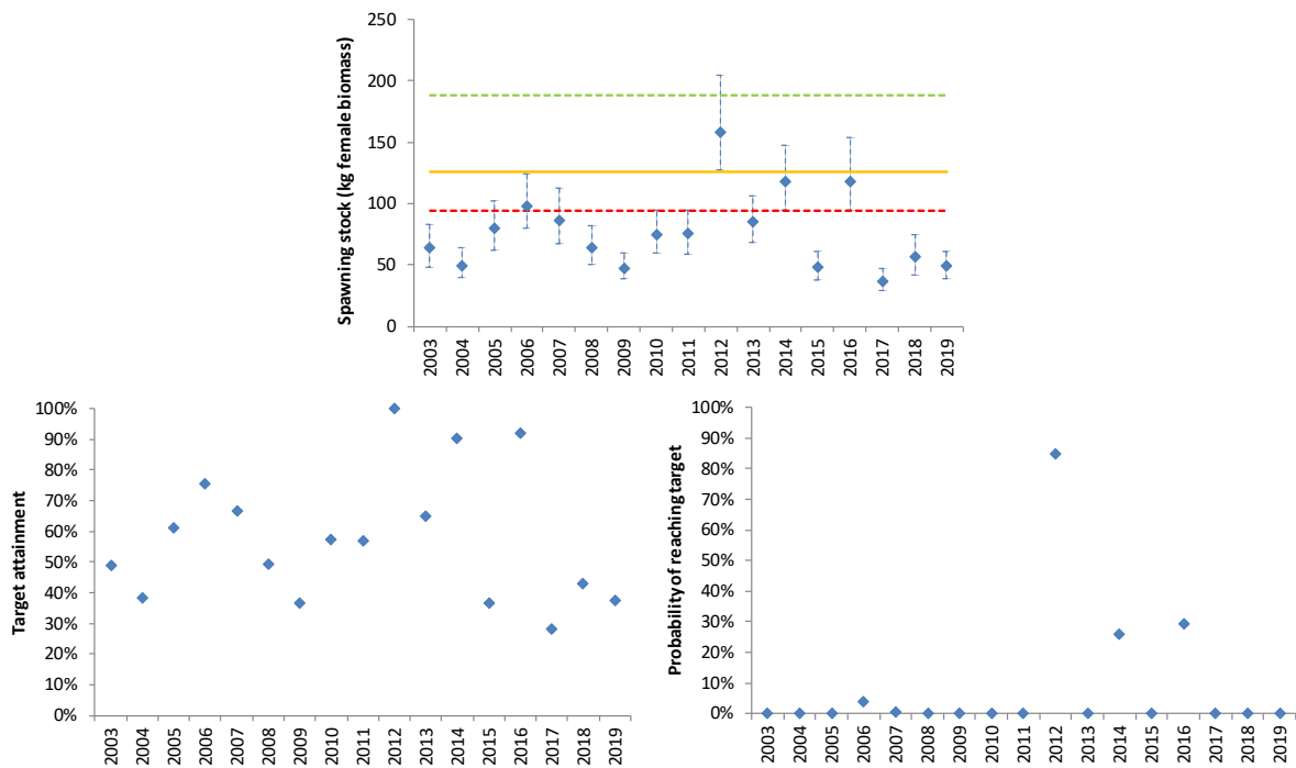
Figure 44. The estimated spawning stock (top row), percent truncated spawning target attainment (bottom row, left) and probability of reaching the spawning target (bottom row, right) in the period 2003-2019 in the Finnish tributary Áhkojohka/Akujoki.
