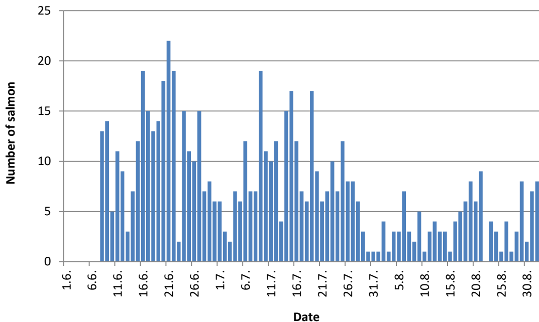
Figure 16. Estimated daily numbers of ascending salmon (≥45 cm) in the River lešjohka between 4.6. and 2.9.2019. All size categories are combined. The estimate of the total ascendance through the site was 656 salmon.
