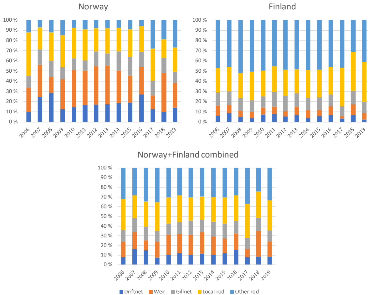
Figure 21. The distribution of catch between fishing gear in the two respective countries (top) and Norway and Finland combined (bottom) in the period 2006-2019.
