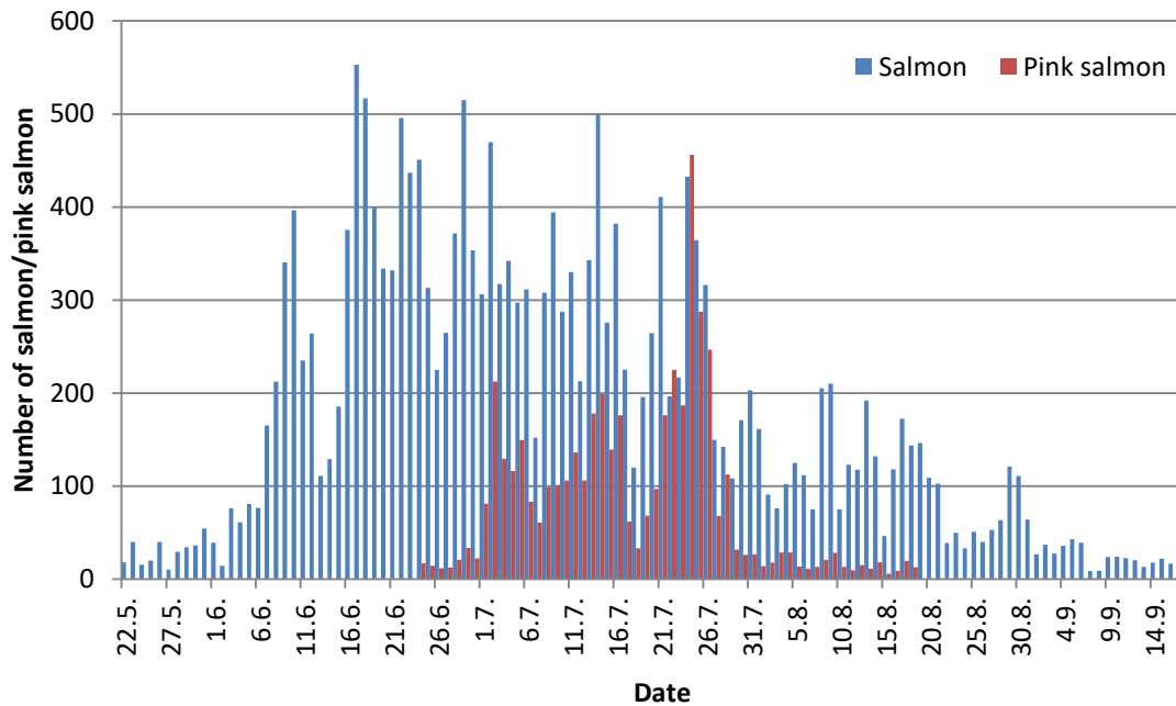
Figure 17. Estimated numbers of salmon (21 013) and pink salmon (4 593) in the Tana/Teno main stem sonar count in 2019. Separation of salmon and pink salmon is based on length frequency data of sonar count and catch data from the nearby river area. Note: the pink salmon numbers are most probably minimum estimates, as only fish larger than 45 cm were measured from the sonar data.
