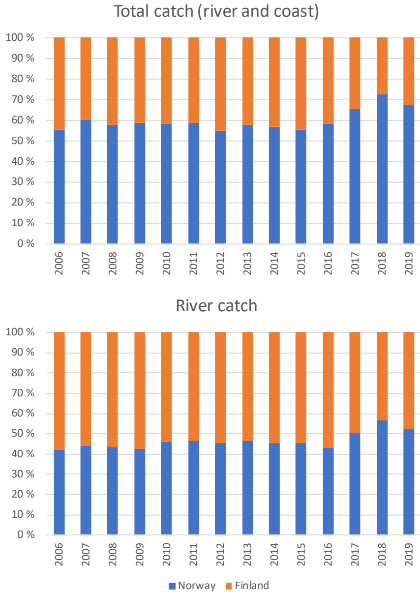
Figure 19. Distribution of catch of Tana/Teno salmon between Norway and Finland for the years 2006-2019. The top graph shows the total catch distribution, with coastal and river catch combined, while the bottom graph shows river catch distribution only.
