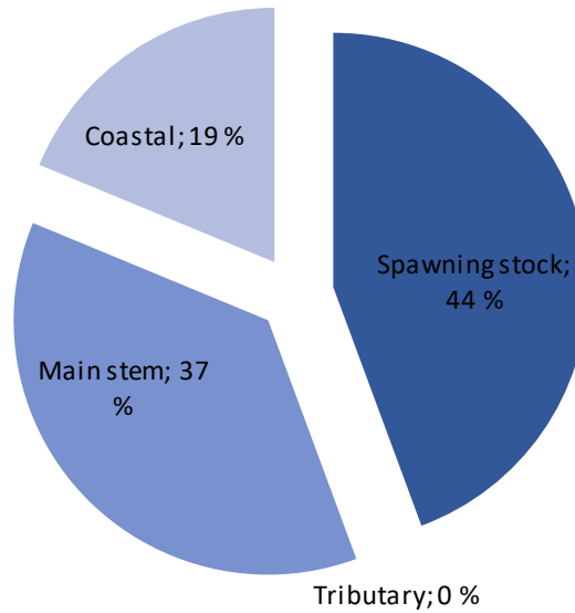
Figure 41. The total amount of salmon belonging to Njiljohka/Nilijoki in 2016-2019, distributed into surviving spawning stock and salmon caught in fisheries in either coastal, main stem or Njiljohka/Nilijoki fisheries. The percentages in the figure represent the proportion of the pre-fishery abundance that survives to spawning or are caught in coastal, main stem or tributary fisheries.
