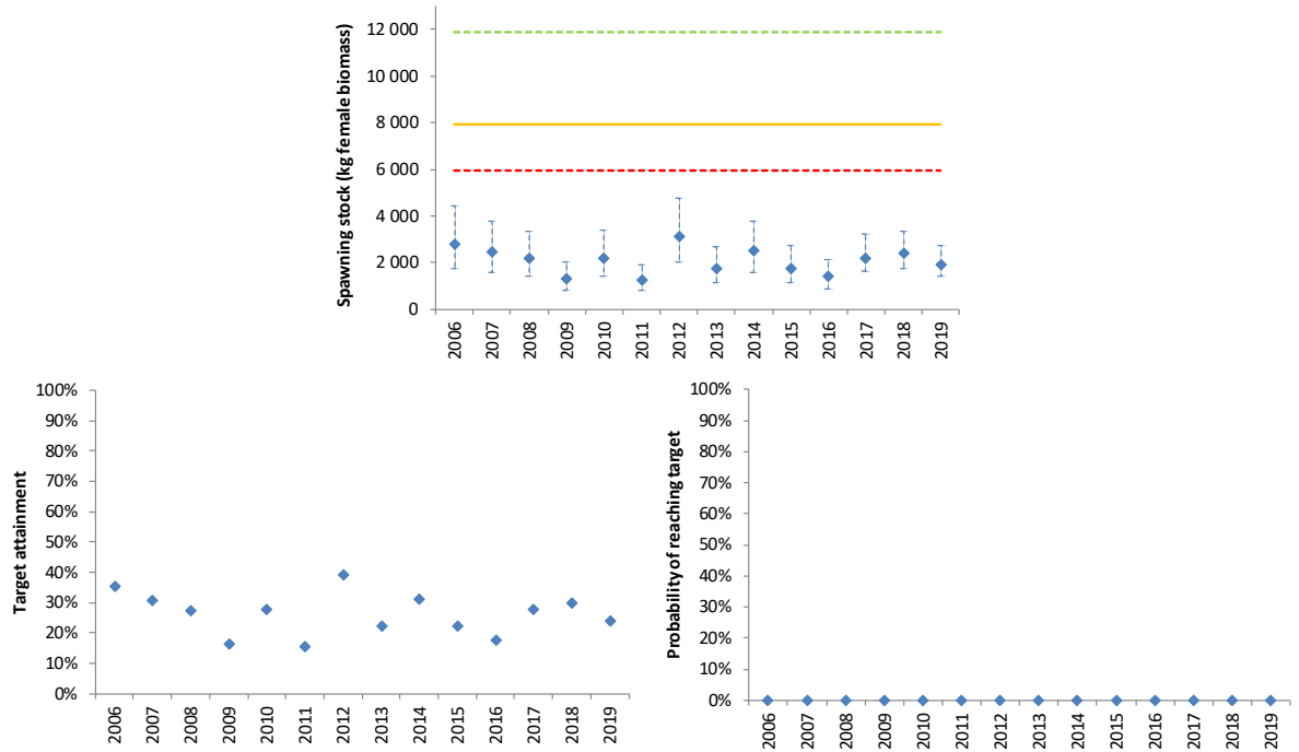
Figure 50. The estimated spawning stock (top row), percent truncated spawning target attainment (bottom row, left) and probability of reaching the spawning target (bottom row, right) in the period 2006-2019 in the tributary Anárjohka/Inarijoki.
