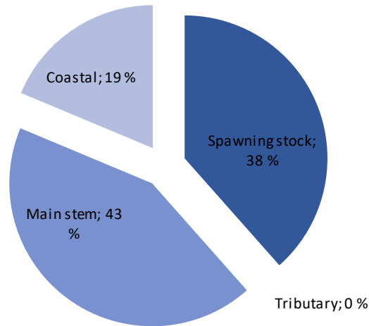
Figure 45. The total amount of salmon belonging to Áhkojohka/Akujoki in 2016-2019, distributed into surviving spawning stock and salmon caught in fisheries in either coastal, main stem or Áhkojohka/Akujoki fisheries. The percentages in the figure represent the proportion of the pre-fishery abundance that survives to spawning or are caught in coastal, main stem or tributary fisheries.
