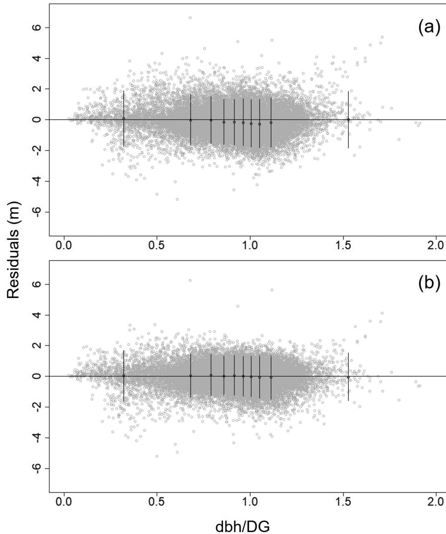
Fig. 3. Residual plots of Näslund's Model 1 (a) and Model 2 (b) against the social status of a tree, dbh/DG to predict tree height of hybrid aspen ( Populus tremula \times P. tremuloides ) in southern Finland. The selected variables and formulas are provided in Eqs. 11 and 12 for Model 1 (a), and Eqs. 13 and 14 for Model 2 (b). Note that here the residual analysis was performed only with fixed-effect parameters for general purposes. The whiskers were offered by the lmfor package in R statistical software to detect any bias (Mehtätalo 2015).
