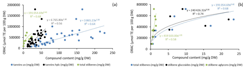
Figure 9. Oxygen radical absorbance capacity (ORAC) of Norway spruce bark (saw logs) as a function of total amounts of condensed tannins and stilbenes (a) and stilbene glycosides and aglycons (b) as analyzed by HPLC, UV and GC-MS methods during storage treatments in 2017.
