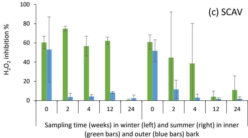
Figure 8. Oxygen radical absorbance capacity (ORAC; a), ferric ion reducing antioxidant power (FRAP; b), and hydrogen peroxide ( H_2O_2 ) scavenging activity (SCAV; c) in inner and outer bark of Norway spruce saw logs after 70% ethanol (70% EtOH) extraction during storage treatments during winter and summer in 2017.
