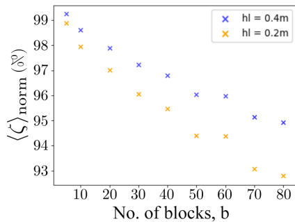
Figure 9. Sensitivity of the average WTD to a difference in the block head level, hl. The values of \langle \zeta^{(b)} \rangle_{\text{norm}} correspond to the optimal block positions computed for hl = 0.2 m (orange) and hl = 0.4 m (blue). The larger the blocks are, the higher the WTD has risen.
