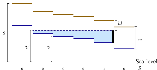
Figure 4. Side view of a canal. The solid blue and the brown horizontal lines represent the initial CWL, v , and the height of the peat surface, s , respectively. The parameter w denotes the distance from the peat surface to the CWL. Each pixel is represented by one line segment. The vertical black line represents the block, and the dotted blue line represents the CWL after the block has been placed, v' . The shaded blue area represents the change in the CWL due to the block. The value of the vector k is k_i = 1 if there is a block in pixel i and otherwise k_i = 0 .
