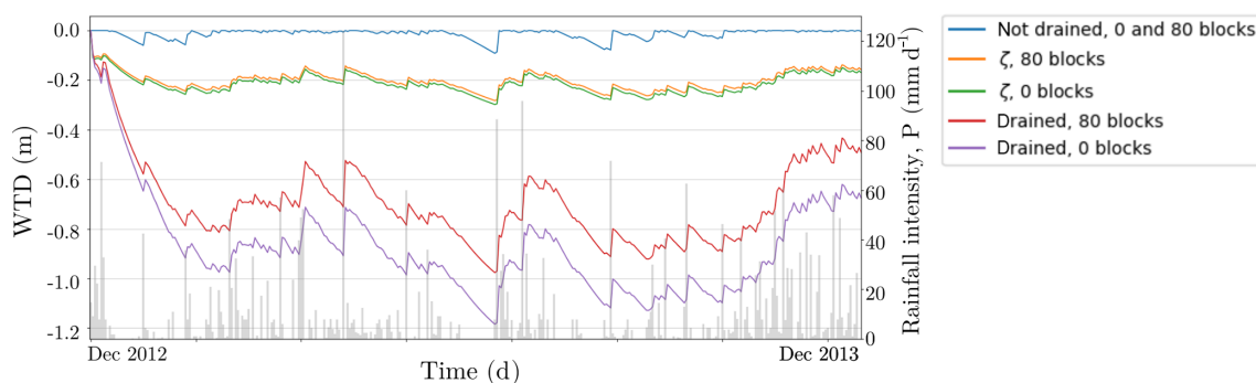
Figure 10. Simulated daily WTD for two sites (drained and natural, see Fig. 7 for the exact locations) within the peatland area and the average WTD, \zeta . The same period (December 2012–December 2013) was simulated without any blocks (green and purple lines) and with the 80 optimized blocks (orange and red lines). The spatial average \zeta for b = \{0, 80\} is shown in orange and green. There was no appreciable difference in WTD in the undrained area between different block configurations, and the WTD is shown by a single line (blue line). Daily rainfall intensity is shown as gray vertical lines (data from Pekanbaru airport).
