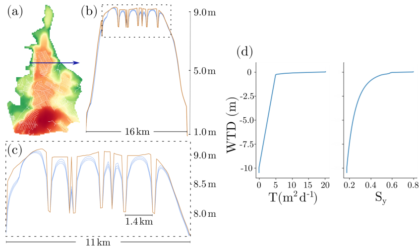
Figure 5. Cross section of the simulated WTD for 3 consecutive dry days after a big rainfall event and peat hydraulic properties. (a) DEM (colored) with the canal network superposed (white) and a straight horizontal blue line indicating the location of the cross section shown in panels (b) and (c). (b) Peat surface (brown) and cross-sectional view of the WTD (blue) measured in meters above sea level. The multiple blue lines correspond to the WTD for the 3 consecutive days of dry down. Abrupt low peat surface values correspond to canals. The dashed rectangle shows the region magnified in the panel below. (c) Magnified area from the panel above. (d) Transmissivity, T(h) , and specific yield, S_y(h) , functions for the deepest substrate (10 m) hemic peat.
