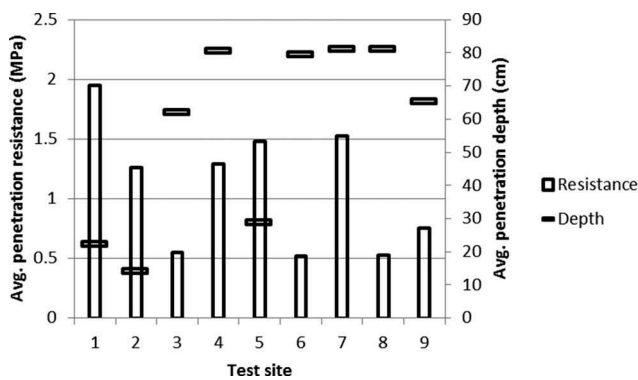
Figure 5. Average penetration resistance of the 20 cm top layer of mineral soil and average maximum penetration depth on the test sites.
