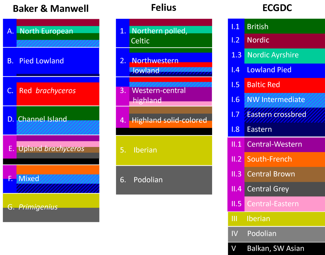
Figure 10. Comparison of the biochemical classification from Baker and Manwell [13], the integrated classification from Felius [2] and the microsatellite-based classification of the European Cattle Genetic Diversity Consortium (ECGDC). The horizontal color bars indicate the groups of the genetic classification. Even colors denote clusters of breeds that are more related to each other than to breeds of other clusters. Hatched colors denote groups of neighboring intermediate or crossbred breeds. The horizontal blocks at the left containing the numbering indicate the five main genetic types of cattle: northern European (blue); central European (violet); Iberian (ochre); Podolian (grey); and Balkan with Anatolian (black).
