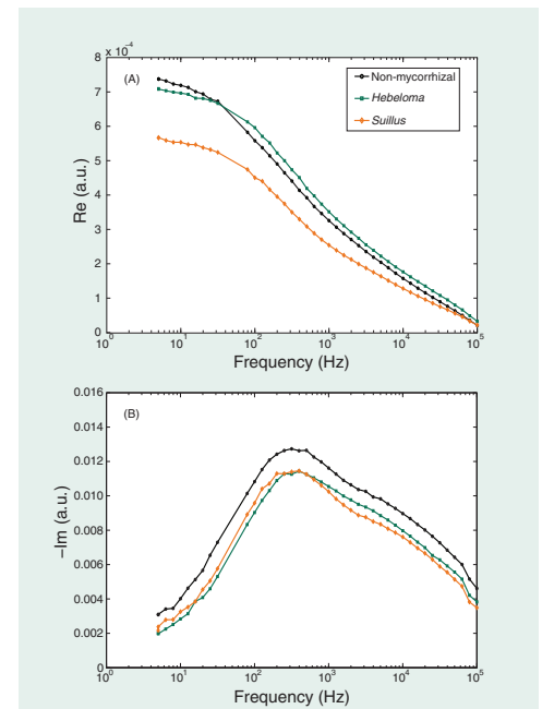
Fig. 3. The normalized real (A) and imaginary (B) part of roots by mycorrhizal treatments (mean of 24 spectra)
