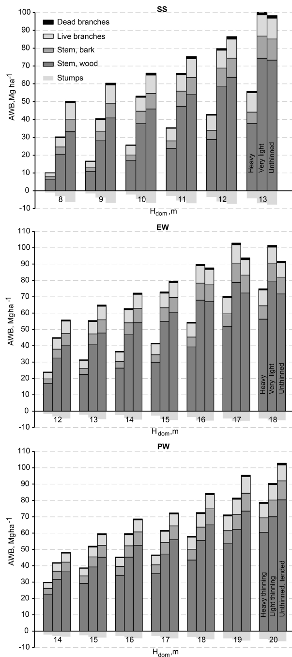
Fig. 5. Mean above-ground woody biomass (AWB) development + stumps of growing stock in downy birch stands by dominant height and treatment in height classes: SS=sapling stand stage, EW=energy wood thinning stage, and PW=pulp wood thinning stage. Dominant height was used as the covariate in Eq. 1, and the models were formulated, and the biomass estimates calculated, through consideration of the mean dominant height separately for each height class at each measurement.
