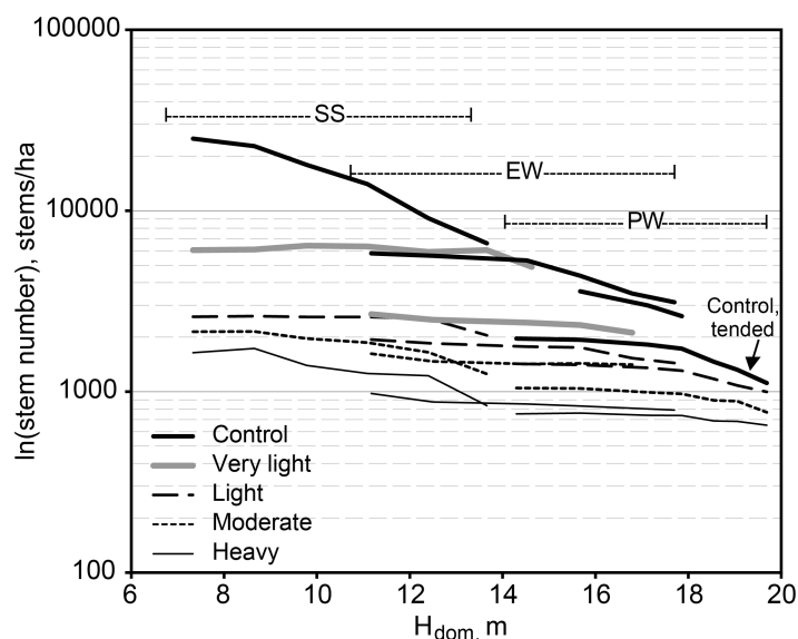
Fig. 1. The mean stem number (on a logarithmic scale) of live trees by first thinning intensity and dominant height during the study period, when the thinning was carried out at the sapling stand stage (SS), at the energy wood thinning stage (EW), and at the pulp wood thinning stage (PW).
