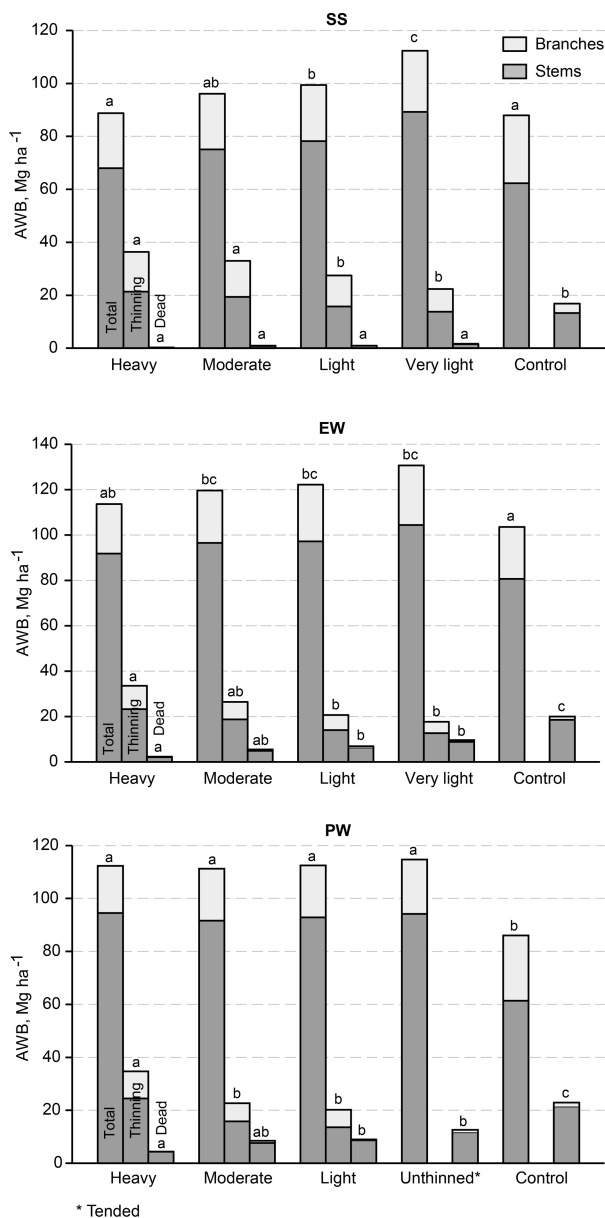
Fig. 6. Estimates of above-ground woody biomass (AWB) production until the end of the study period for different initial thinning intensities in height classes: SS=sapling stand stage, EW=energy wood thinning stage, and PW=pulp wood thinning stage. The total AWB figures include live trees in the final growing stock and in first-thinning removal. Treatments denoted with the same letter (within a height class) are not significantly different ( p > 0.05 ). Site index, H_{50} , and dominant height at final measurement were used as the covariates in Eq. 1 for total production, and their mean values for each height class (SS: H_{50} = 14.1 and H_{dom} = 12.9 m, EW: H_{50} = 17.2 and H_{dom} = 17.6 m, PW: H_{50} = 15.4 and H_{dom} = 19.0 m) were used in calculation of the estimated means. No covariate was used in models of the removal in thinnings, but the length of the study period was considered in the modelling of mortality: mean period 25 years for EW and PW, 22 years for SS.
