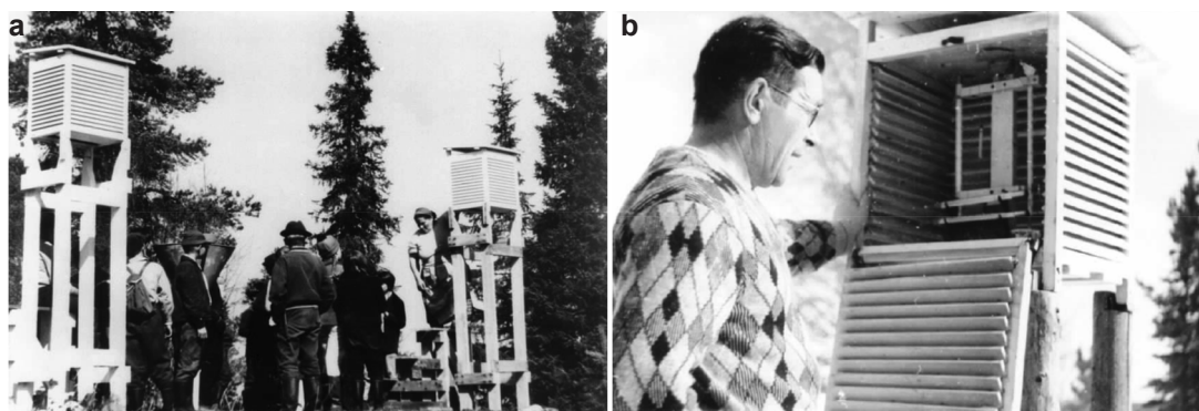
Fig. 2. (a) Mrs. Esteri Pakasmaa (née Kotakorva) making meteorological observations at the Pallasjärvi weather station in 1963. Local school children are following the procedure. (b) Mr. Viljo Pakasmaa beside the instrument shelter at Pallasjärvi in 1965. The shelter contains a thermometer to measure the ambient temperature, a wet-bulb thermometer for obtaining the dew point of the air, and a minimum–maximum thermometer for daily minimum and maximum temperatures. Photos: Ms. Sofia Pyykönen's family album via Pallastunturi Nature Centre.
