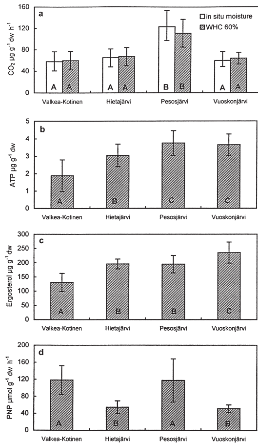
Fig. 2. Soil respiration (a), ATP content (b), ergosterol content (c), and acid phosphatase activity (d) of the soil samples (dw). Standard deviations marked on bars. Bars indexed with different letters (A, B, or C) were significantly different between study areas ( p < 0.001 ).
