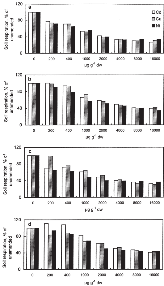
Fig. 3. The soil respiration rate (expressed as a percentage of the rate in unamended soil) of the Cd, Cu and Ni soil samples from Valkea-Kotinen (a), Hietajärvi (b), Pesosjärvi (c), and Vuoskojärvi (d).
