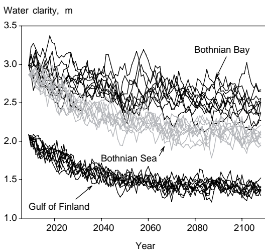
Fig. 4. Ten baseline projections for average water clarity in the three basins.
