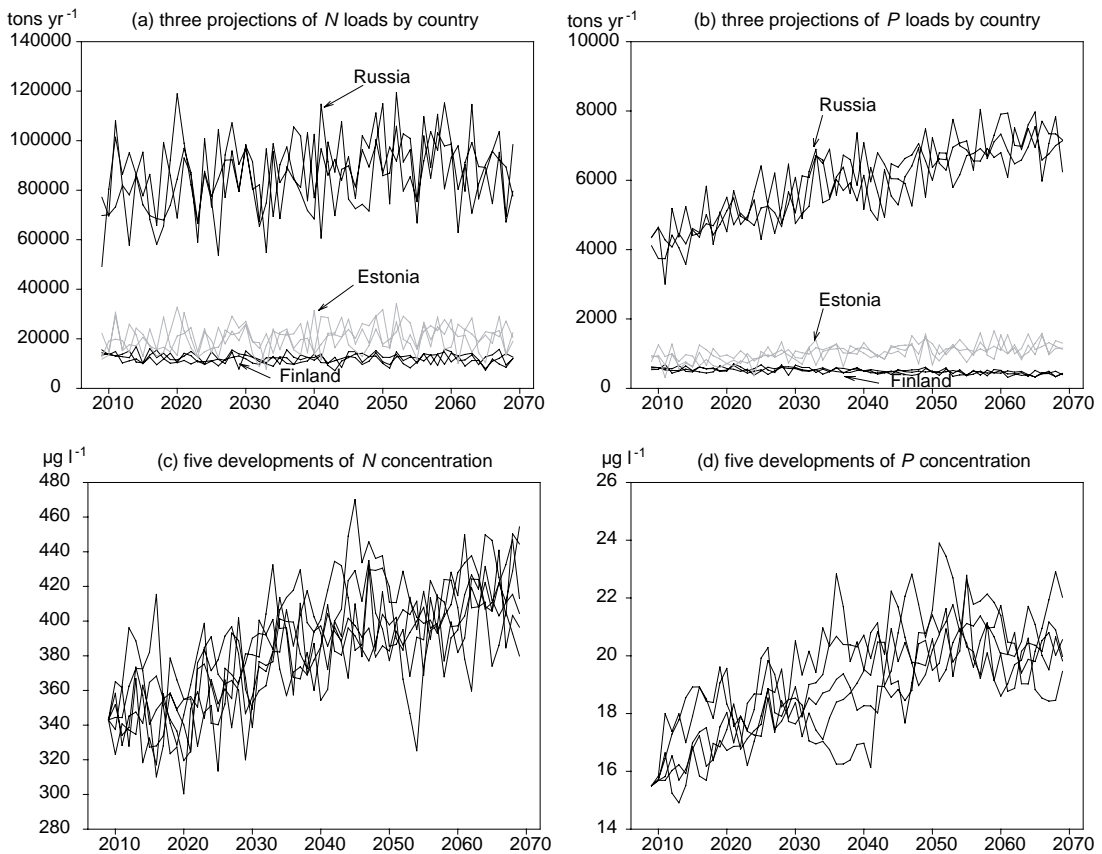
Fig. 2. Baseline projections of land loads and developments of nutrient concentrations over the next 60 years in the Gulf of Finland.
