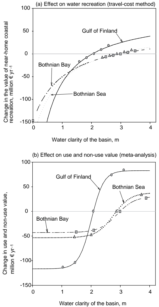
Fig. 3. The effect of altered water clarity
