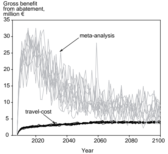
Fig. 5. Ten sample paths for abatement benefits in the Gulf of Finland for a 30% reduction in P loads. Assumption: All countries in the northern Baltic Sea reduce nutrient loads in the same proportion.
