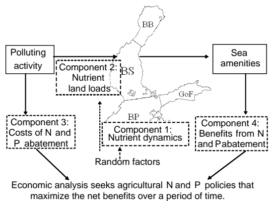
Fig. 1. Framework for the application of economic methods to the management of eutrophication
