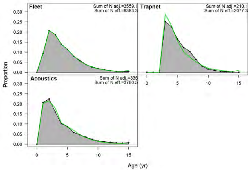
Figure 5. Herring SDs 30-31. Model fits to age composition data.
