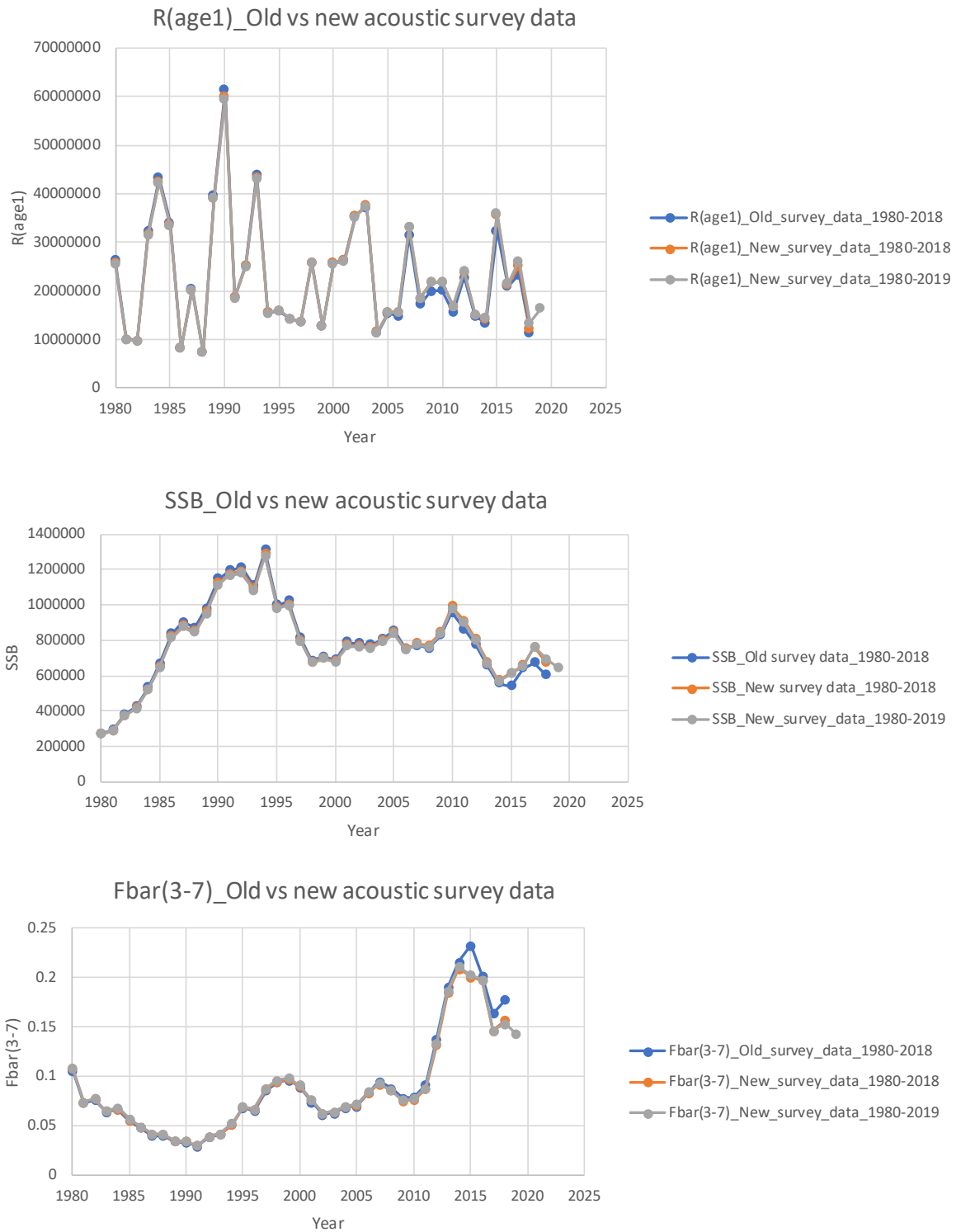
Figure 2. SAM model based estimates of R(\text{age}1) , SSB and F_{\text{bar}}(3-7) using the old and new acoustic survey data.
