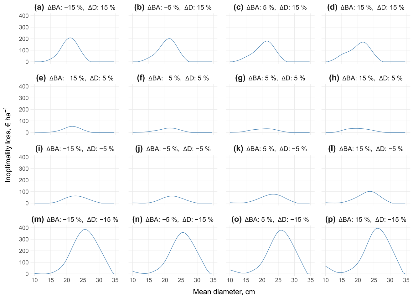
Fig. 4 Inoptimality losses ( \text{€ ha}^{-1} ) as a function of mean diameter when the errors in basal area (BA) and mean diameter ( D ) vary between -15 and 15\% . The mean diameter on the x -axis is the basal
