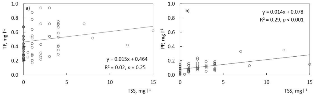
Figure 9a. Relationship between concentrations (mg l -1 ) of total suspended solids (TSS) and a) total phosphorus (TP), b) particulate phosphorus (PP) and c) dissolved reactive phosphorus (DRP) in individual water samples (n = 71) of simulated snowmelt-induced runoff outflow from very fine sandy loam soil during 2011–2013 (Paper II).
