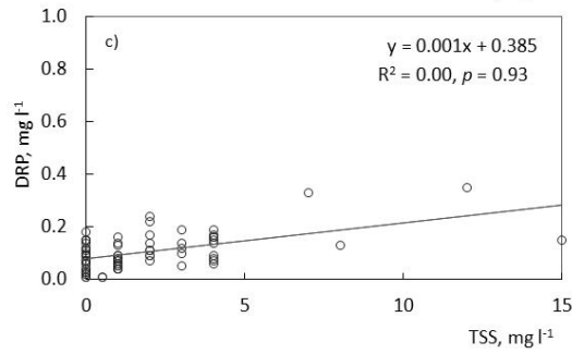
Figure 9a. Relationship between concentrations (mg l -1 ) of total suspended solids (TSS) and a) total phosphorus (TP), b) particulate phosphorus (PP) and c) dissolved reactive phosphorus (DRP) in individual water samples (n = 71) of simulated snowmelt-induced runoff outflow from very fine sandy loam soil during 2011–2013 (Paper II).
