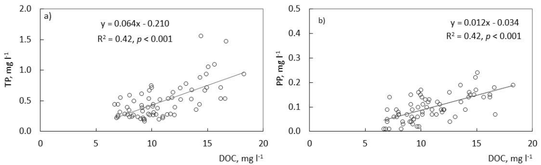
Figure 9b. Relationship between concentrations (mg l -1 ) of dissolved organic carbon (DOC) and a) total phosphorus (TP), b) particulate phosphorus (PP) and c) dissolved reactive phosphorus (DRP) in individual water samples (n = 69) of simulated snowmelt-induced runoff outflow from very fine sandy loam soil during 2011–2013 (Paper II). Note difference in scale of Y-axis.
