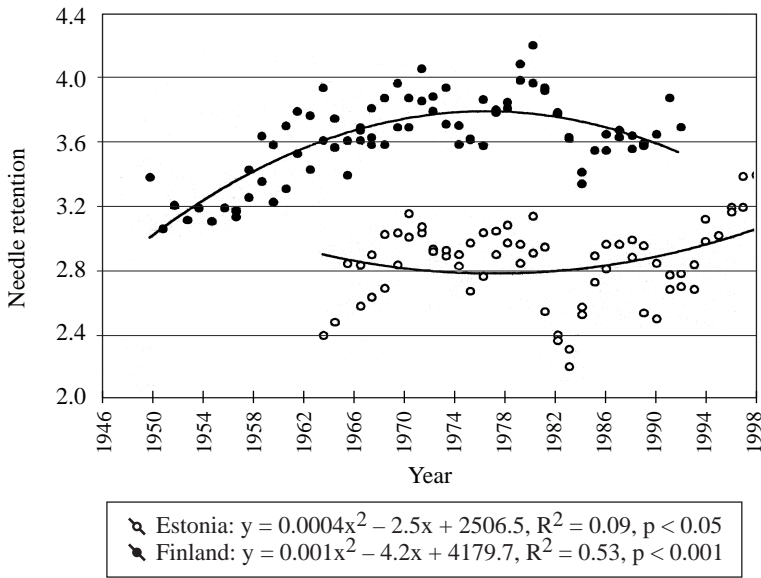
Fig. 2. Long-term changes in needle retention with time.
