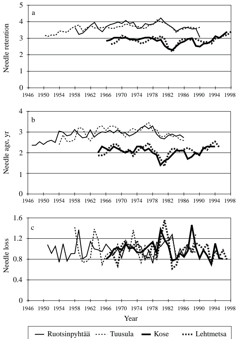
Fig. 1. Needle chronologies on Pinus sylvestris in Kose and Lehtmetsa in northern Estonia, and in Tuusula and Ruotsinpyhtää in southern Finland, a) needle retention; b) needle age; c) needle loss.
