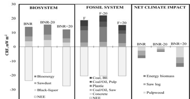
Figure 2. Cumulative radiative forcing, CRF ( \text{mW m}^{-2} ) of different components of the biosystem and the fossil system at the end of the 90-year period in Finland. NEE: net ecosystem \text{CO}_2 exchange, BNR: baseline management with energy wood thinning and harvesting of branches, needles (70%), tops of stems, and stumps and roots from final felling, BNR±20: 20% higher or lower stocking in thinning with harvesting of energy biomass, and F±20: corresponding fossil system (Kilpeläinen et al. 2015).
