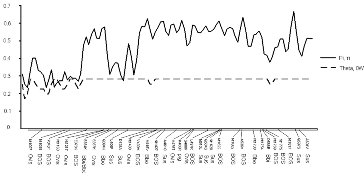
Figure 4 Sliding window presentation of the nucleotide divergence along PRLR exon 10 among 18 different species. \pi = cattle, Bbi = American bison, Bbo = European bison, Ovis = sheep, Sus = pig. The positions of the detected SNPs are shown on the X-axis.
