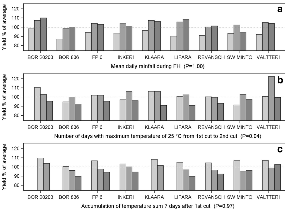
Fig. 3 Yield responses of meadow fescue cultivars ( G \times E ). The dashed line indicates 100 % of the average yields of the cultivars for 2000–2012. P values are for the statistical significance for the interaction between the cultivar and the weather variable. The columns are as follows: low (light gray), moderate (medium gray) and high (dark gray) accumulation of a mean daily rainfall during FH, b number of days with the maximum temperature of 25 °C from the first cut to the second cut and c temperature sum 7 days after the first cut. For further details regarding the low, moderate and high categories, see Table 2
