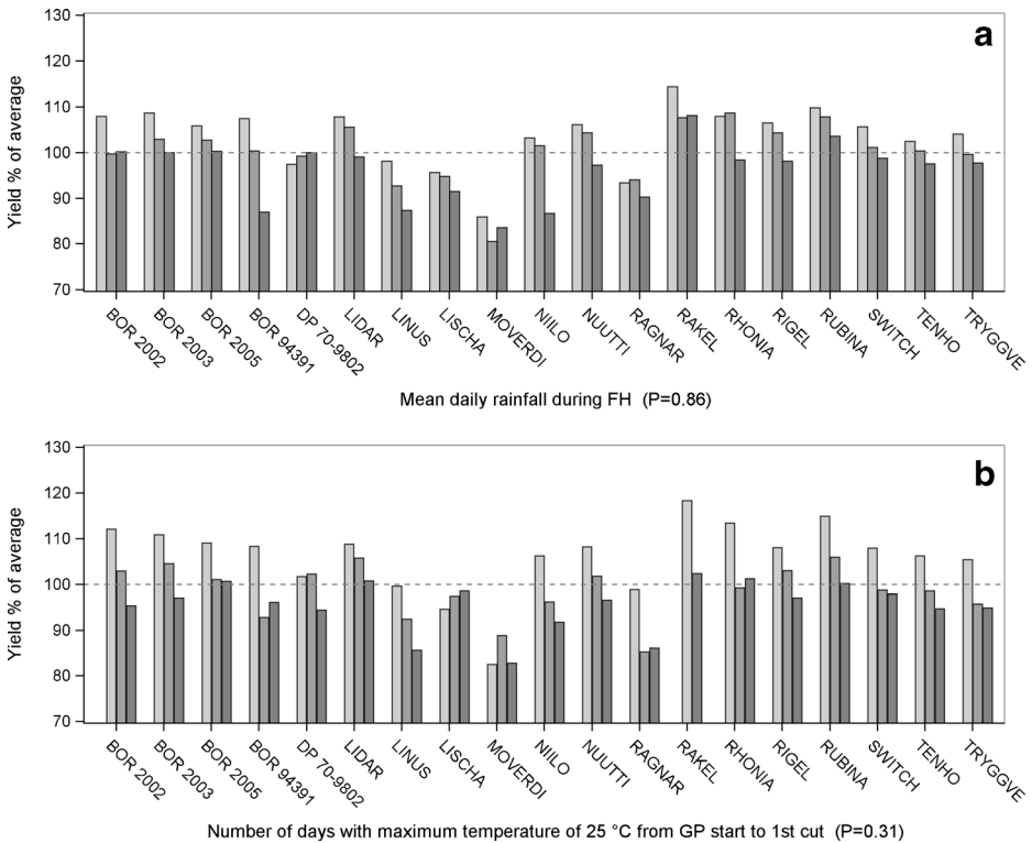
Fig. 2. Yield responses of timothy cultivars (G \times E). The dashed line indicates 100 % of the average yields of the cultivars for 2000–2012. P values are for the statistical significance for the interaction between the cultivar and the weather variable. The columns are as follows: low (light grey), moderate (medium grey) and high (dark grey) accumulation of a mean daily rainfall during the fall hardening period and b number of days with the maximum temperature of 25 °C from the start of the growth period to the first cut. For further details regarding the low, moderate and high categories, see Table 2
