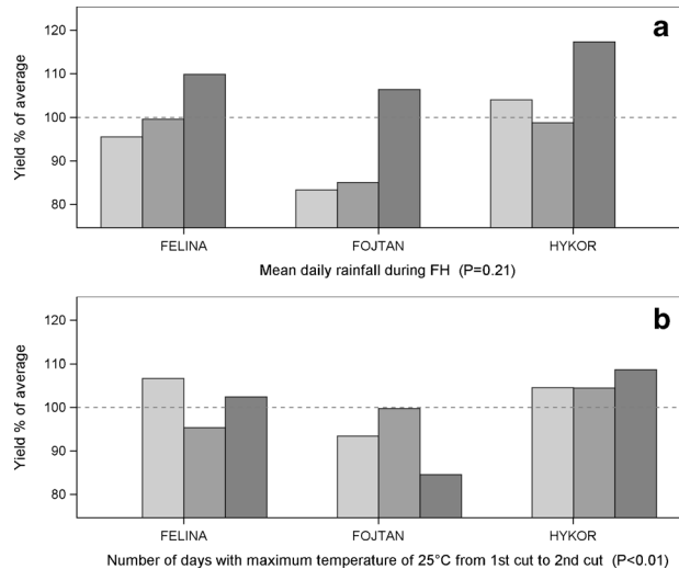
Fig. 5 Yield responses of festulium cultivars (G × E). The dashed line indicates 100 % of the average yields of the cultivars for 2000–2012. P values are for the statistical significance for the interaction between the cultivar and the weather variable. The columns are as follow: low (lightest gray), moderate (medium gray) and high (darkest gray) accumulation of a mean daily rainfall during the FH and b number of days with the maximum temperature of 25 °C from the first cut to the second cut. For further details regarding the low, moderate and high categories, see Table 2
